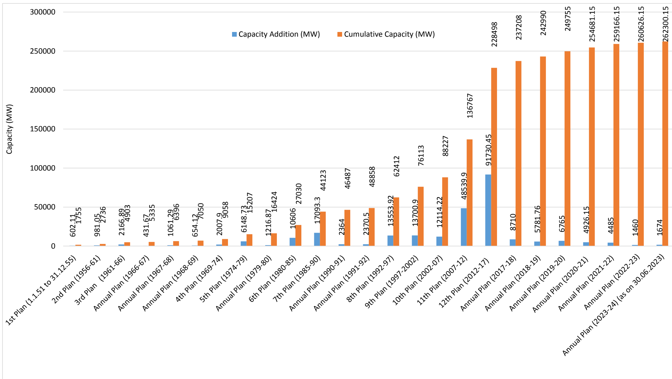
6.0 Bar Chart representing Plan / Year wise Growth of Thermal Capacity in the country (Till 30.09.2023) -
