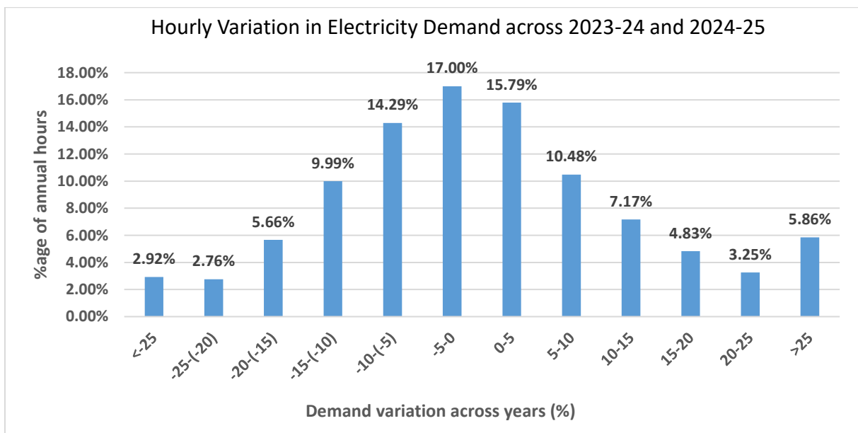
Figure 7: Hourly Variation in Electricity Demand across years
