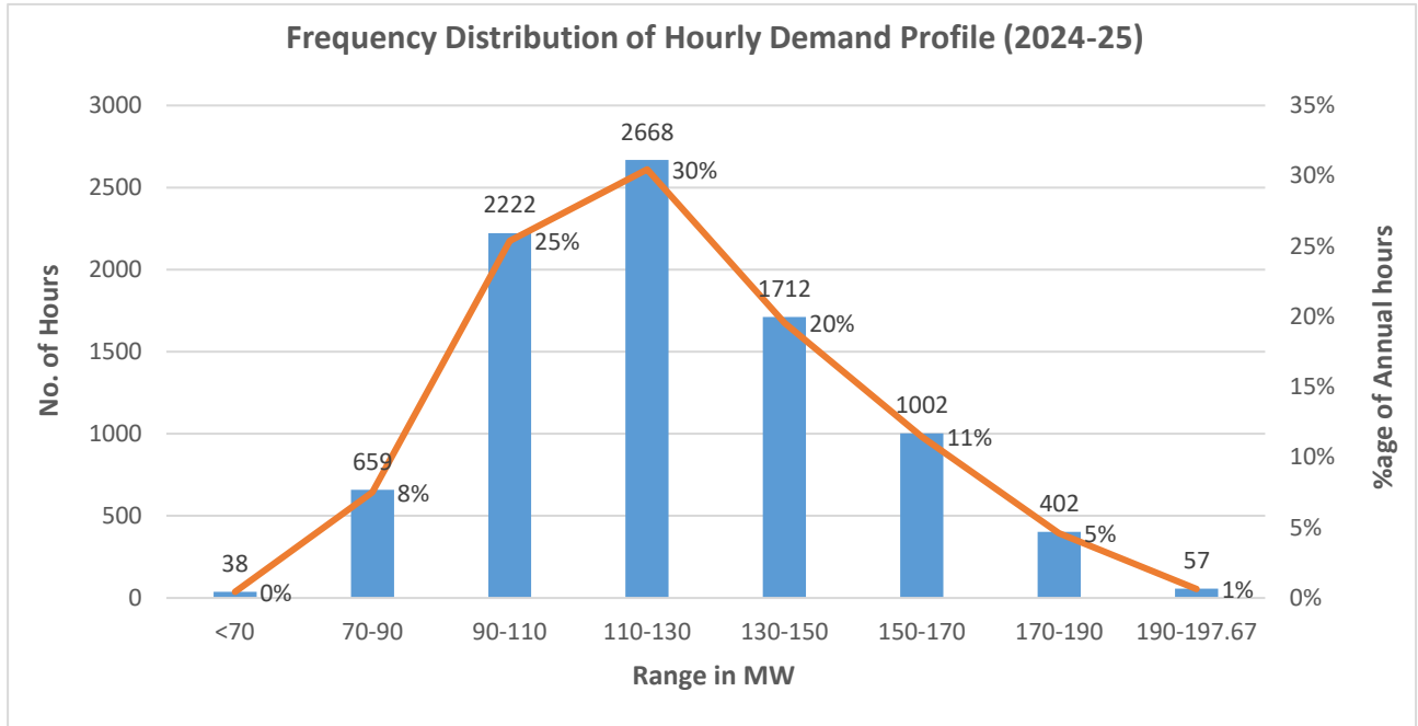
Figure 5: Frequency Distribution of Hourly Demand Profile of 2024-25
