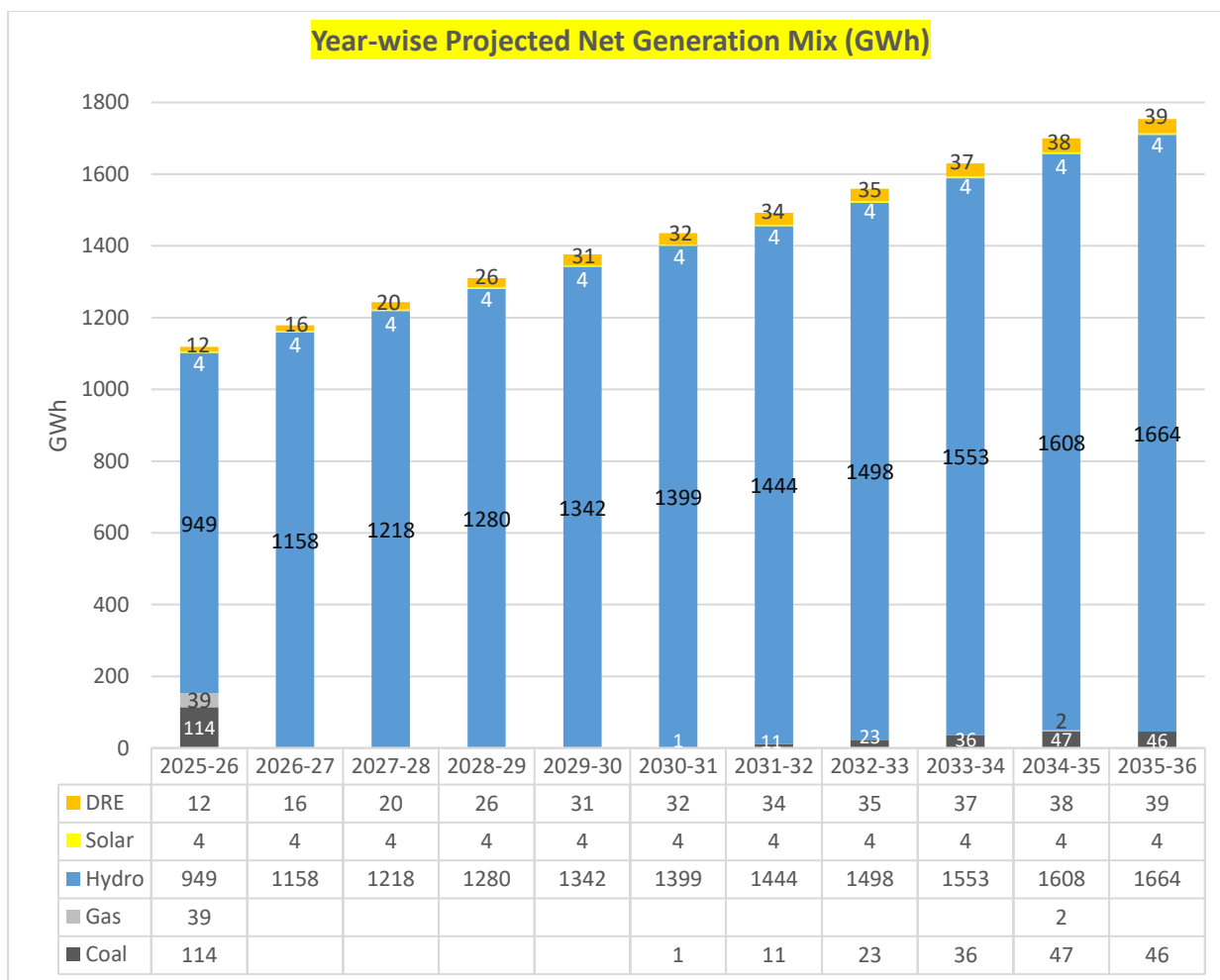
Figure 11: Year-wise projected net generation (in GWh)
