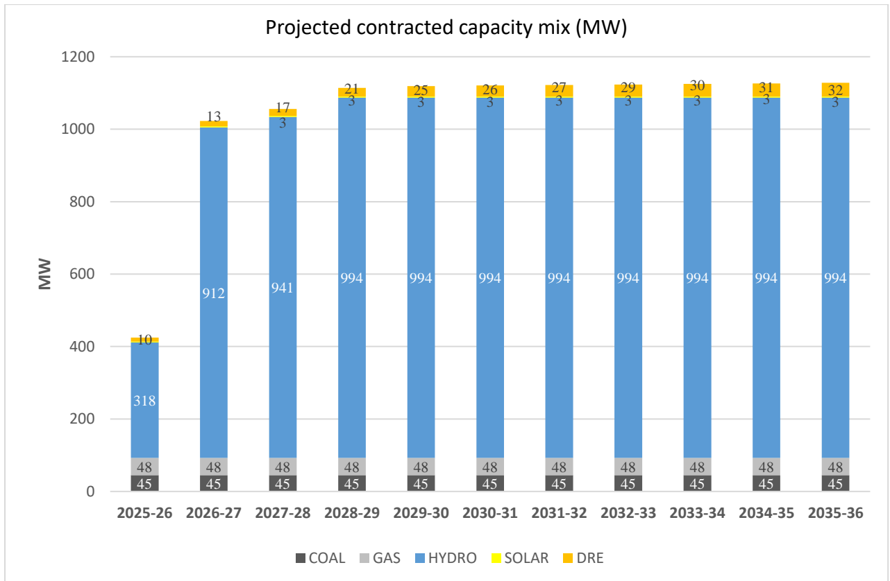
Figure 8: Projected Contracted Capacity Mix Year-wise (MW)
