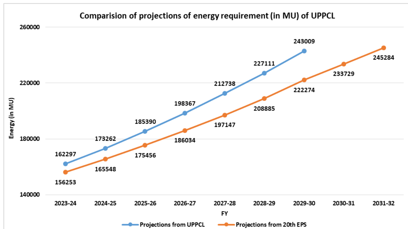
Figure 5 Graph on Energy requirement comparison
