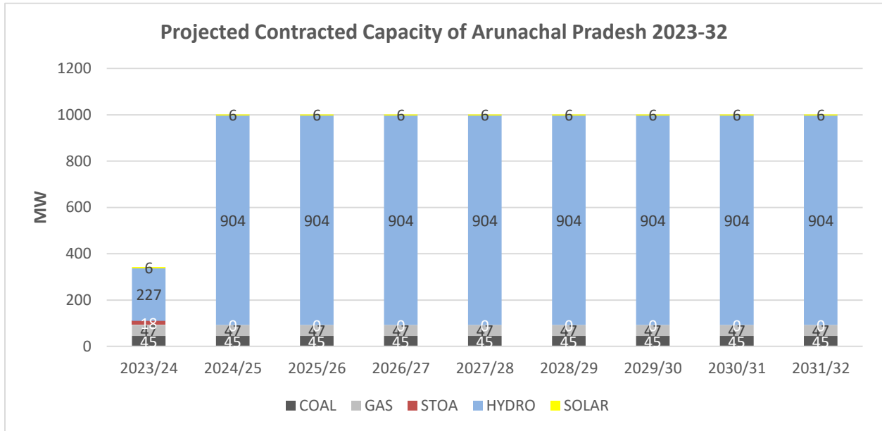
Figure 5 Projected Capacity Mix Year-wise (MW) for Arunachal Pradesh
