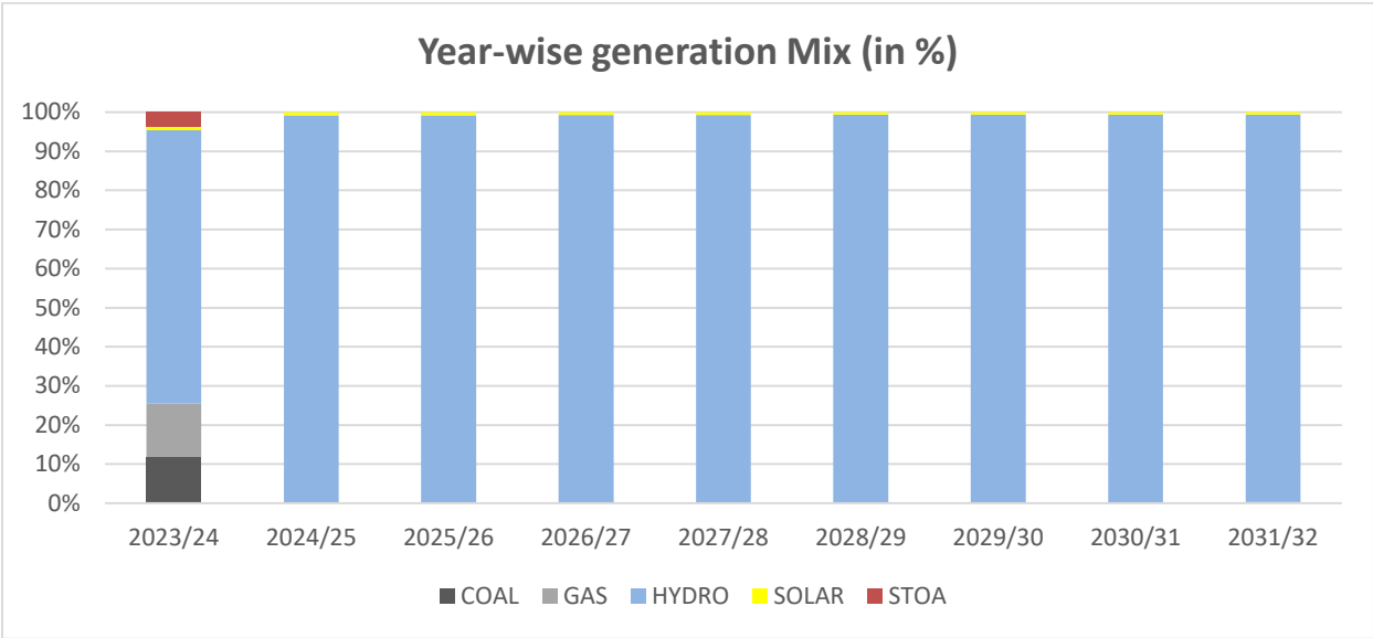
Figure 7 Year-wise projected generation mix (in %age)
