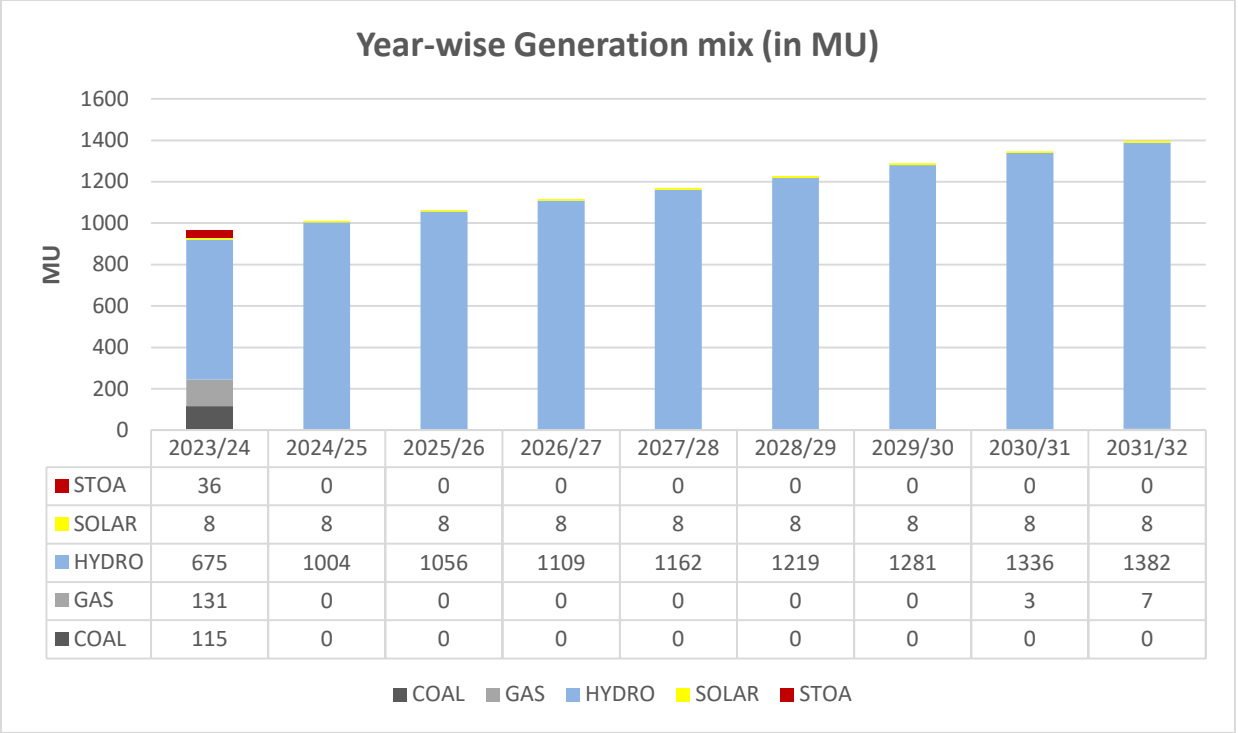
Figure 8 Year-wise projected generation mix (in GWh)
