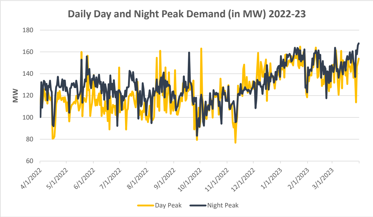
Figure 3 Day and Night Peak in MW of Arunachal Pradesh (2022-23)
