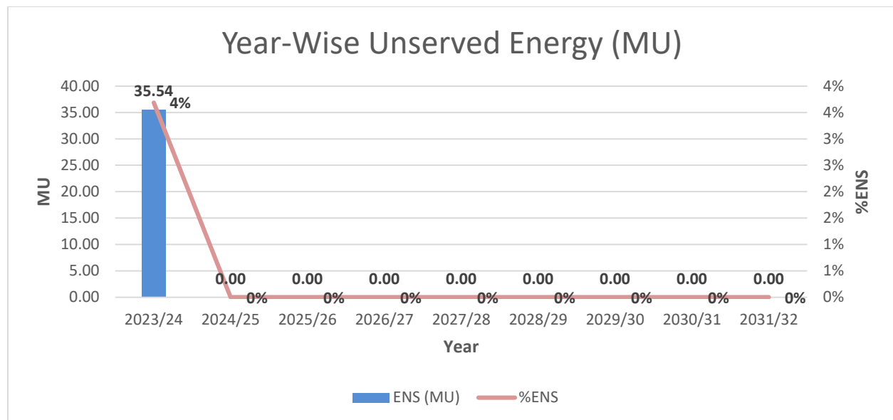
Figure 4 Yearly likely unserved energy with the planned capacities for Arunachal Pradesh (in MU)
