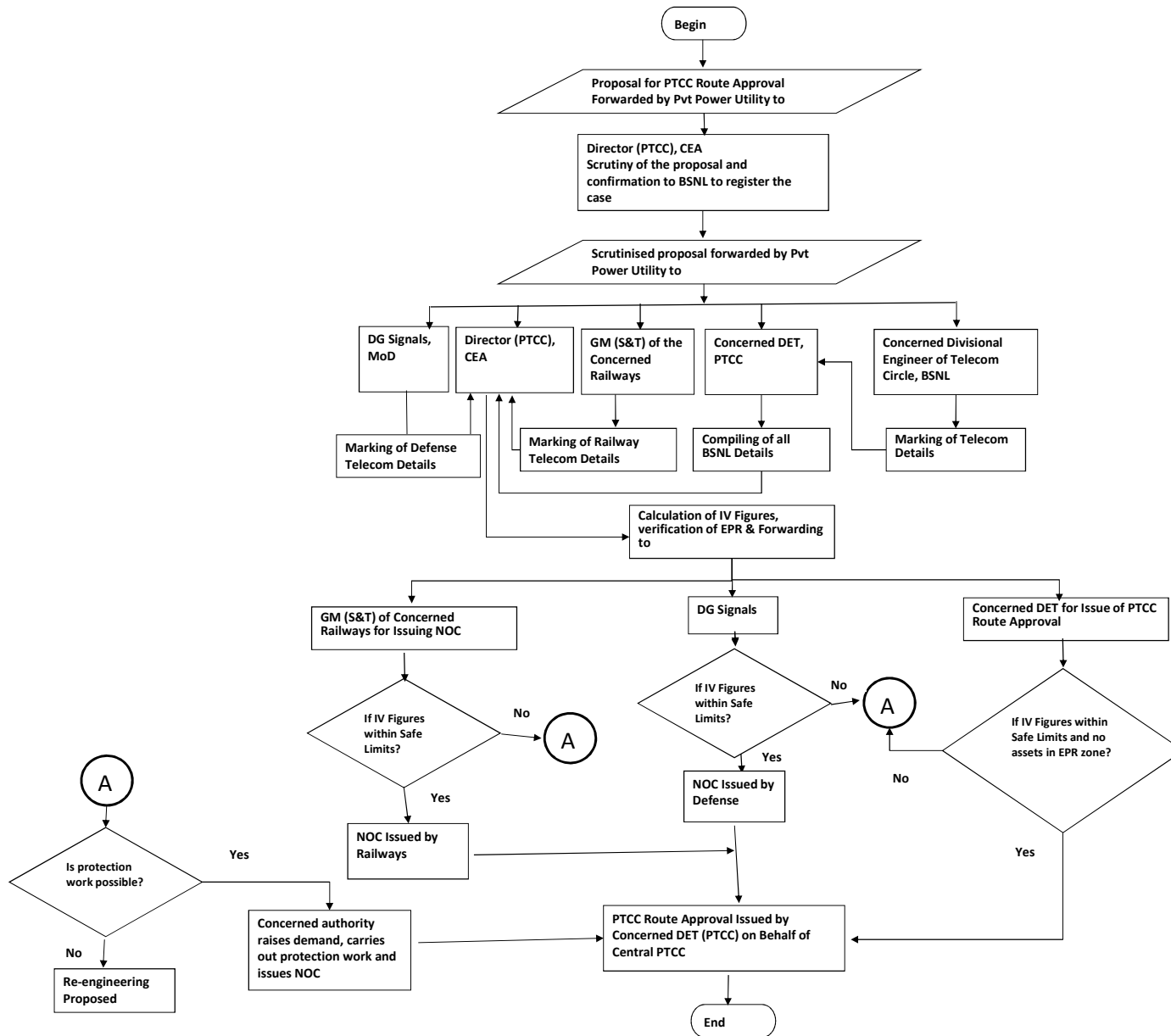
Flow-chart of PTCC Process for 220 kV and above transmission lines of Pvt Power Utility
