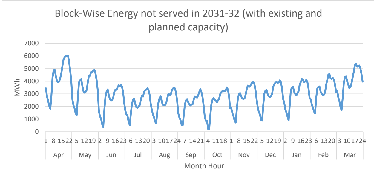
Figure 5 Daily Unserved Energy Pattern MU (2031-32)
