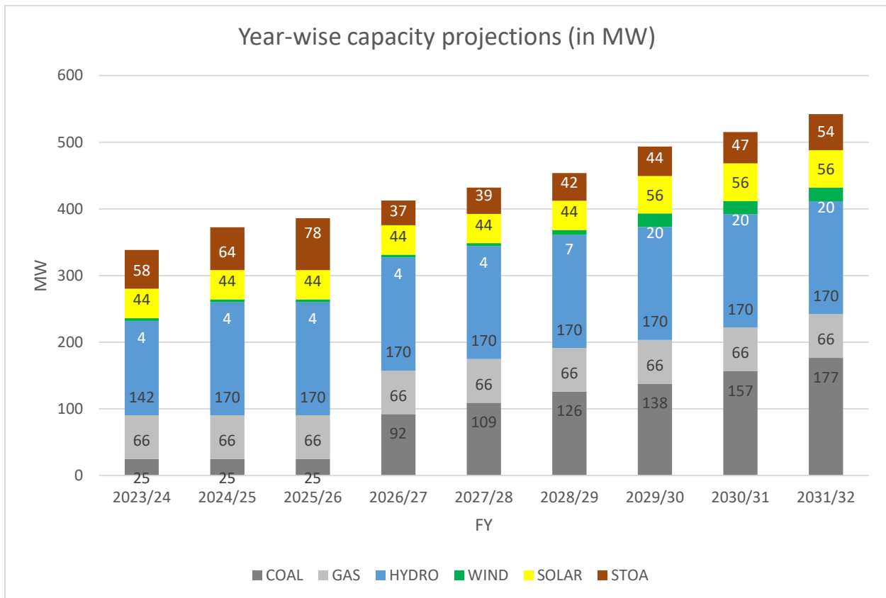
Figure 6 Projected Capacity Mix Year-wise (MW) for Mizoram
