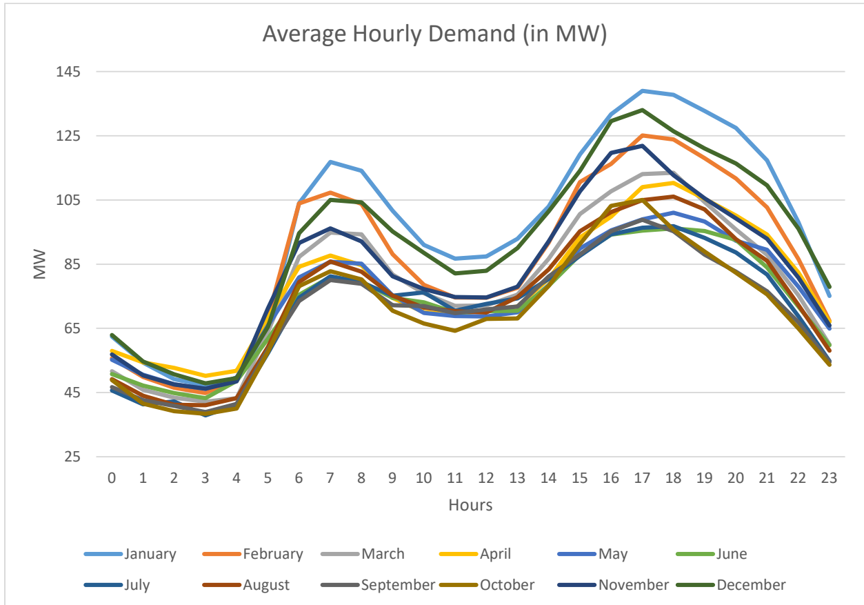
Figure 2 Average Hourly Demand Profile (MW)
