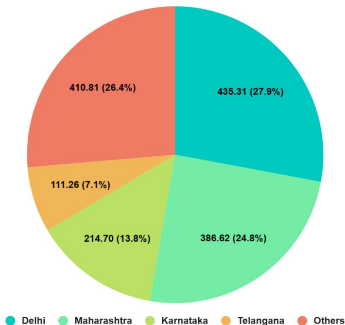
Total EV-PCS Electricity Consumption in 2025-26 (Till Mar 2026) (in MU)
