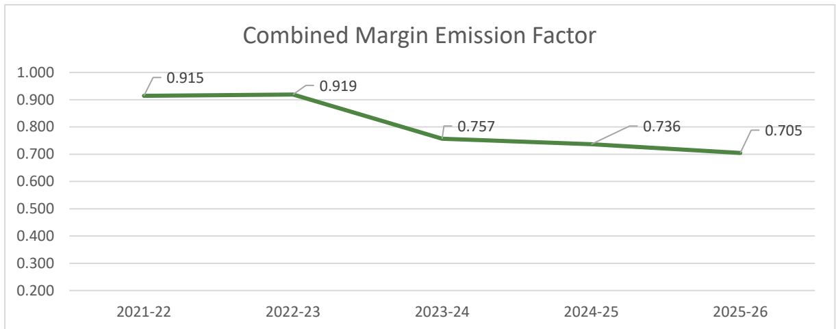
Figure 6: Development of the combined margin (adjusted for electricity transfers) for the Indian Grid over the period 2021-22 to 2025-26.
