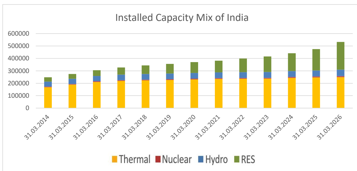
Figure 2: The Installed Capacity Mix of India
