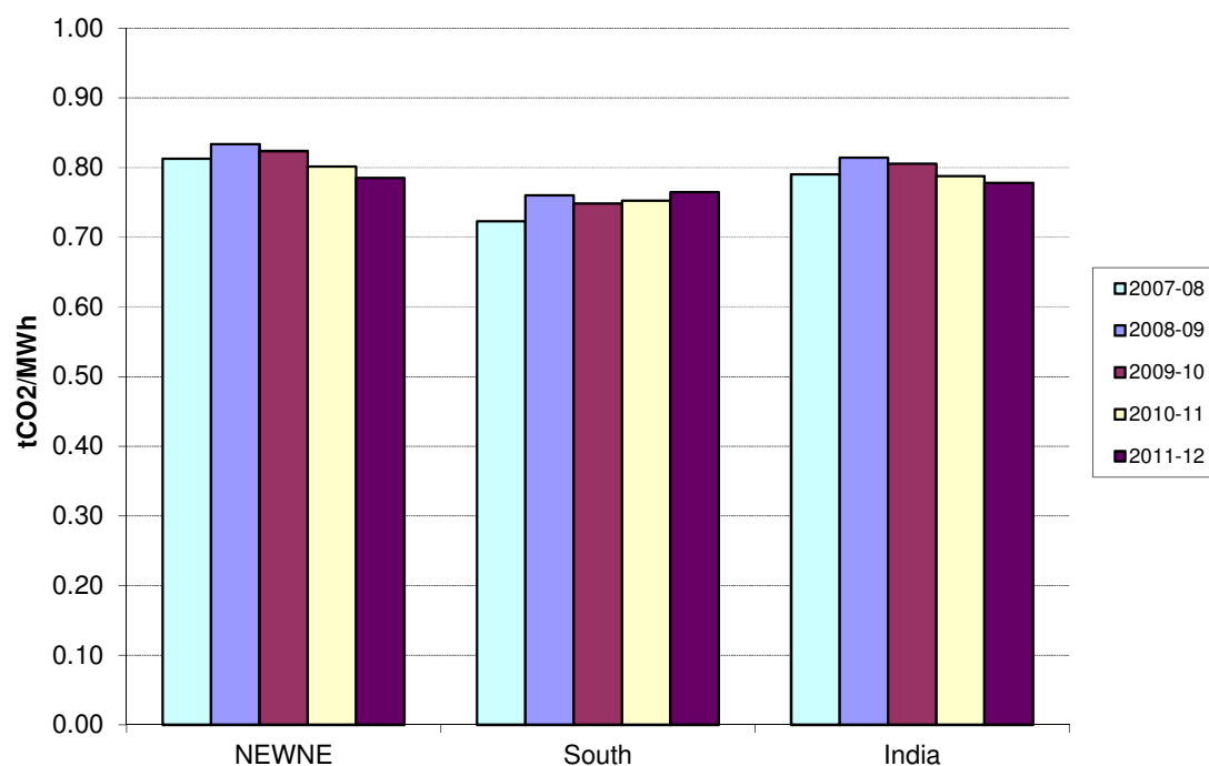
Figure 2: Development of the weighted average emission factor (adjusted for electricity transfers) for India's grids over the period 2007-08 to 2011-12
