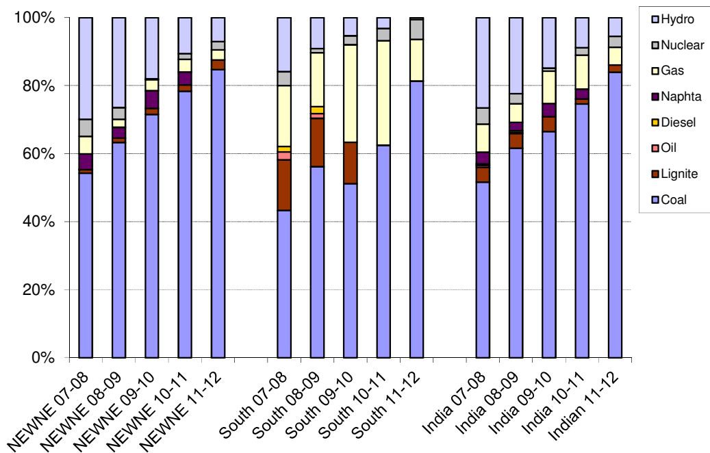
Figure 5: Breakdown of the build margins by fuel type and grid (shares based on net generation)
