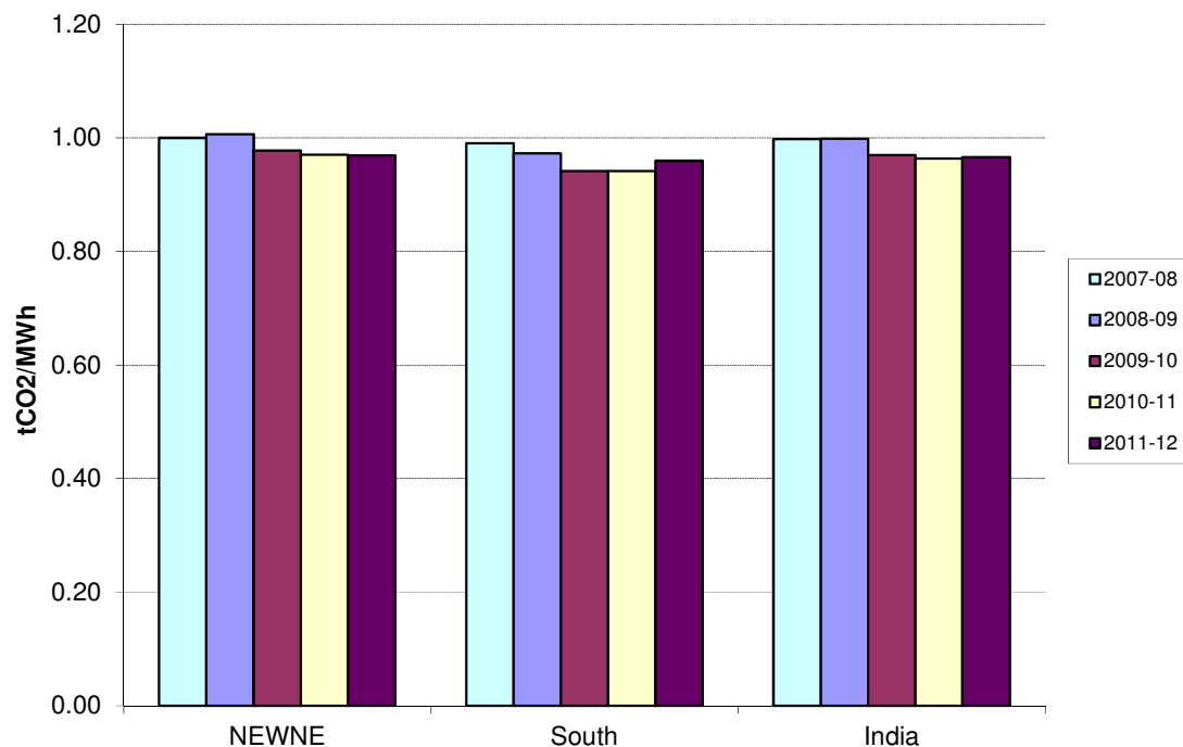
Figure 3: Development of the operating margin (adjusted for electricity transfers) for India's grids over the period 2007-08 to 2011-12
