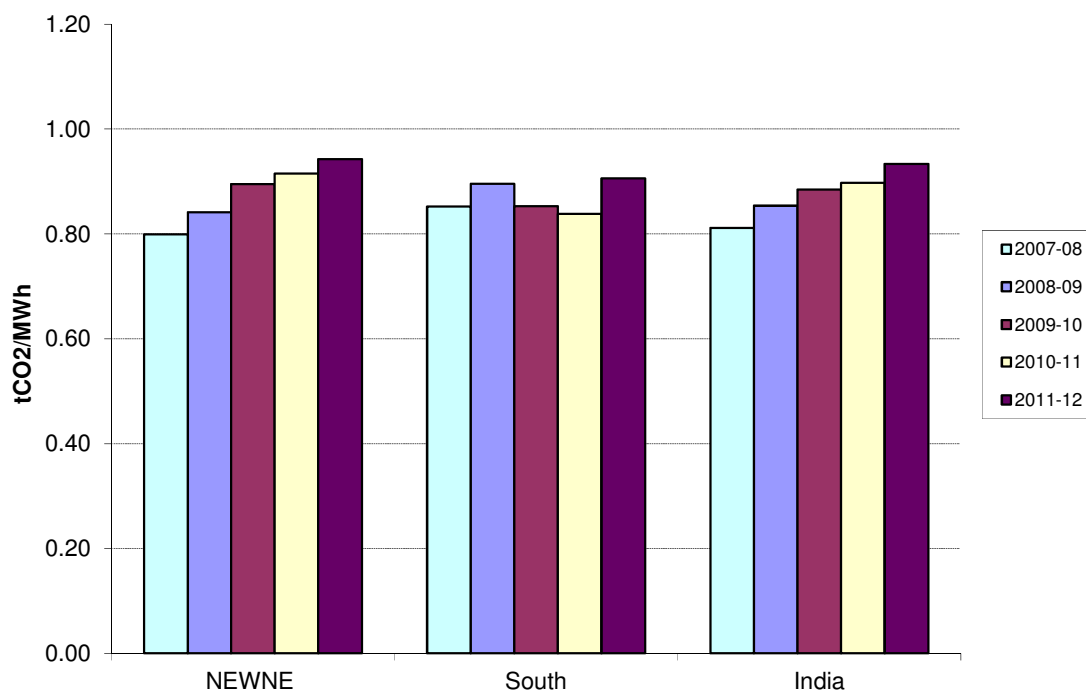
Figure 6: Development of the combined margin (adjusted for electricity transfers) for India's grids over the period 2007-08 to 2011-12
