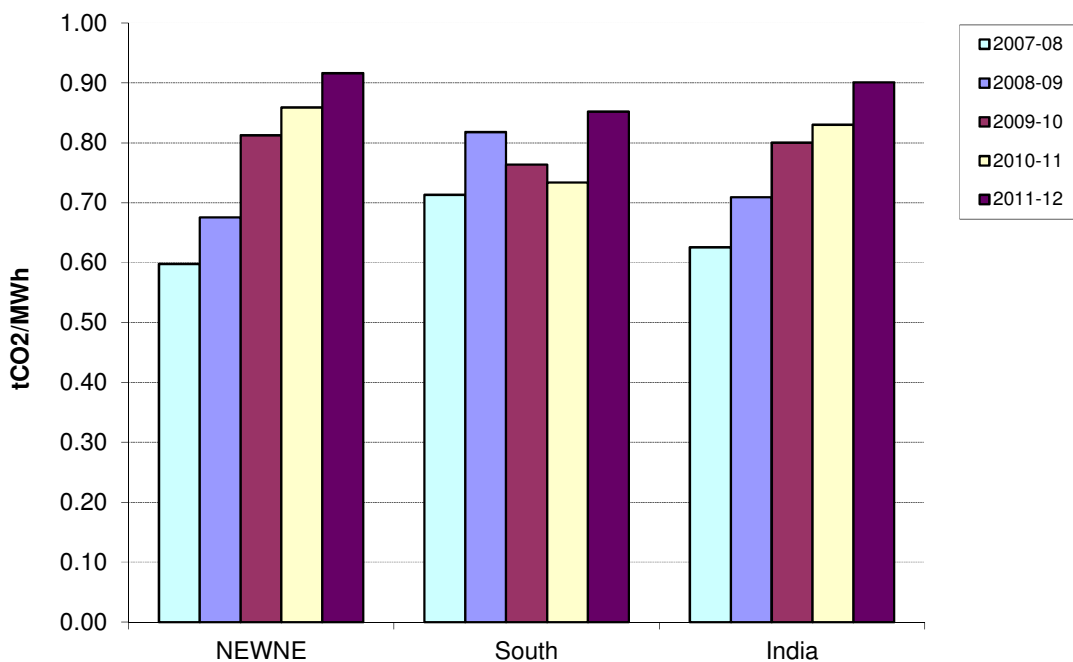
Figure 4: Development of the build margins over the period 2007-08 to 2011-12
