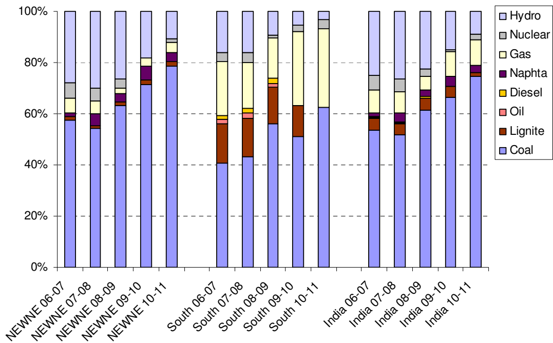
Figure 4: Breakdown of the build margin (comparison of FY 2006-07 to 2010-11) by station and fuel type for grids (shares based on net generation)
