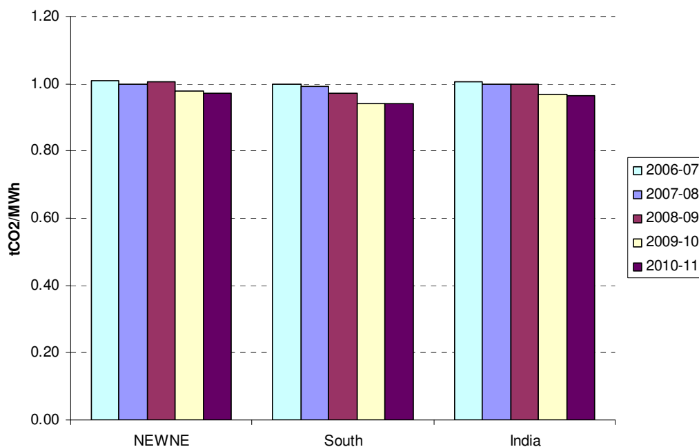
Figure 2: Development of the operating margin (adjusted for electricity transfers) for India's grids over the period 2006-07 to 2010-11.
