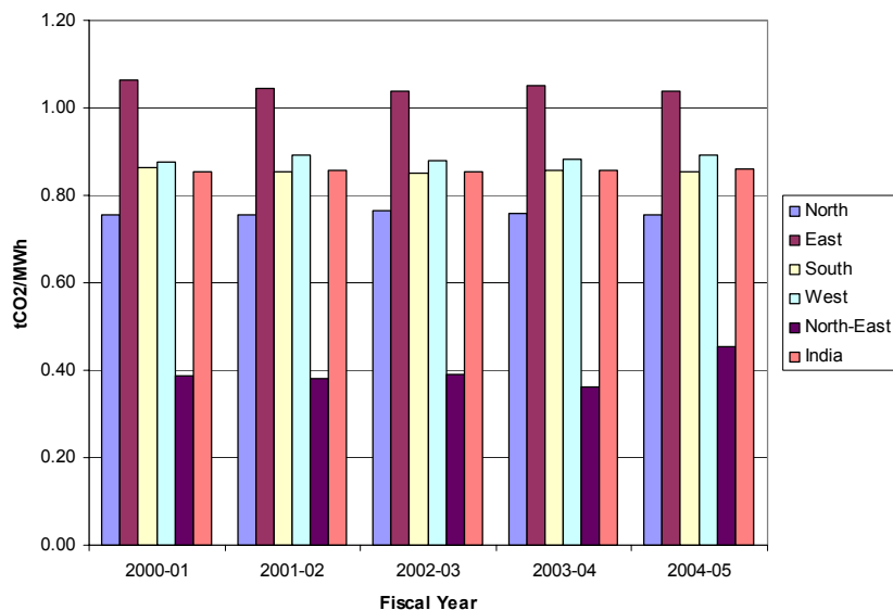
Figure 3: Development of the combined margin (adjusted for electricity transfers) for India's regional grids over the period 2000-01 to 2004-05.
