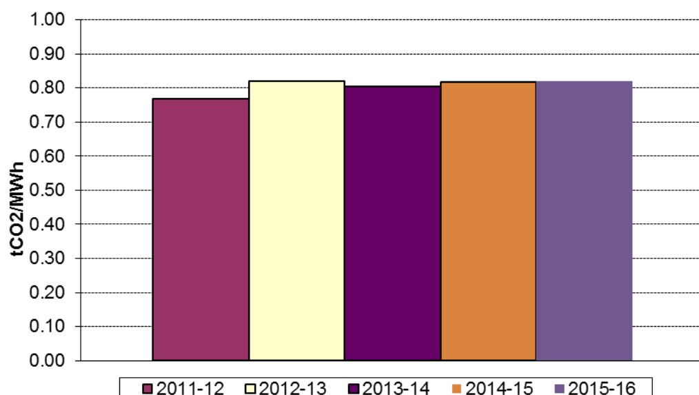
Figure 3: Development of the weighted average emission factor (adjusted for electricity transfers) for the Indian Grid over the period 2011-12 to 2015-16
