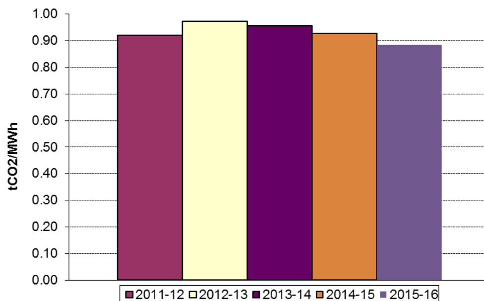
Figure 5: Development of the build margins over the period 2011-12 to 2015-16
