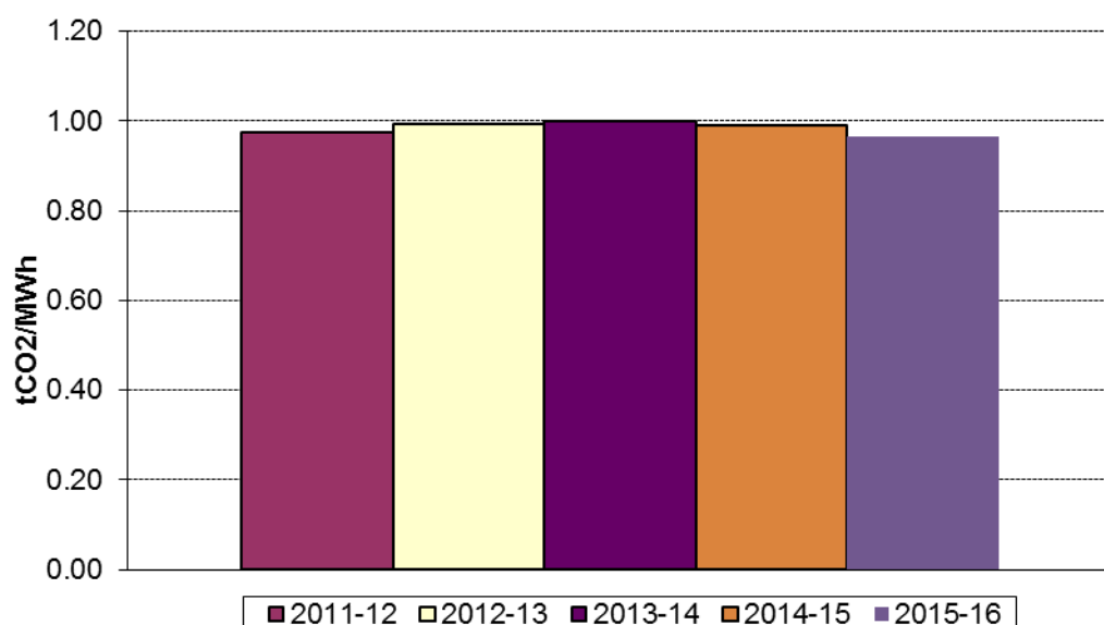
Figure 4: Development of the operating margin (adjusted for electricity transfers) for the Indian Grid over the period 2011-12 to 2015-16
