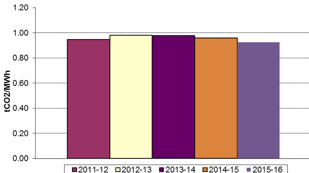
Figure 7: Development of the combined margin (adjusted for electricity transfers) for the Indian Grid over the period 2011-12 to 2015-16
