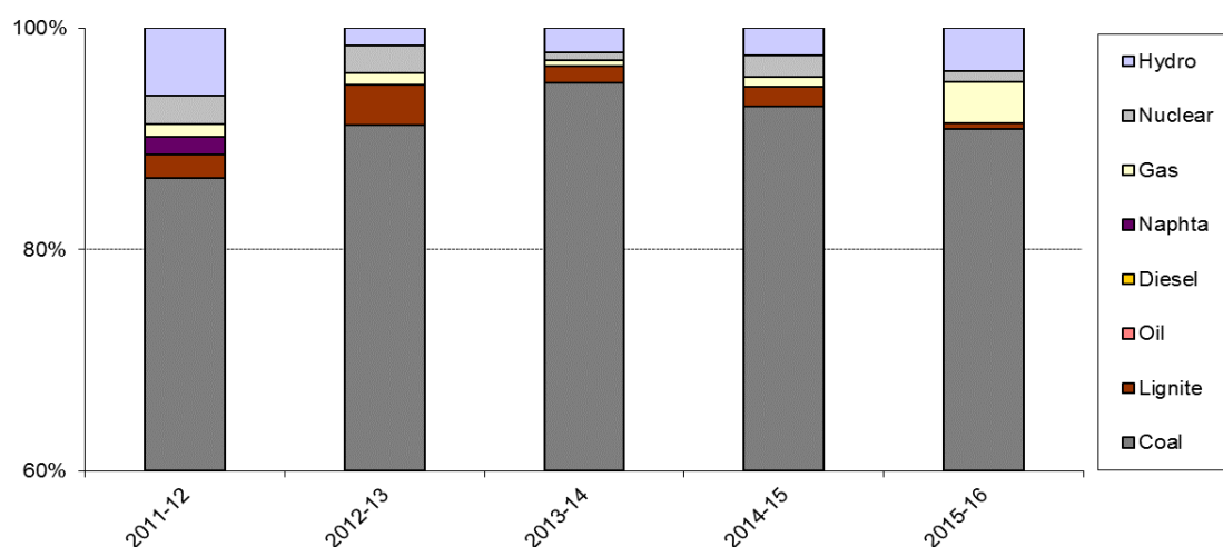
Figure 6: Breakdown of the build margins by fuel type (shares based on net generation)
