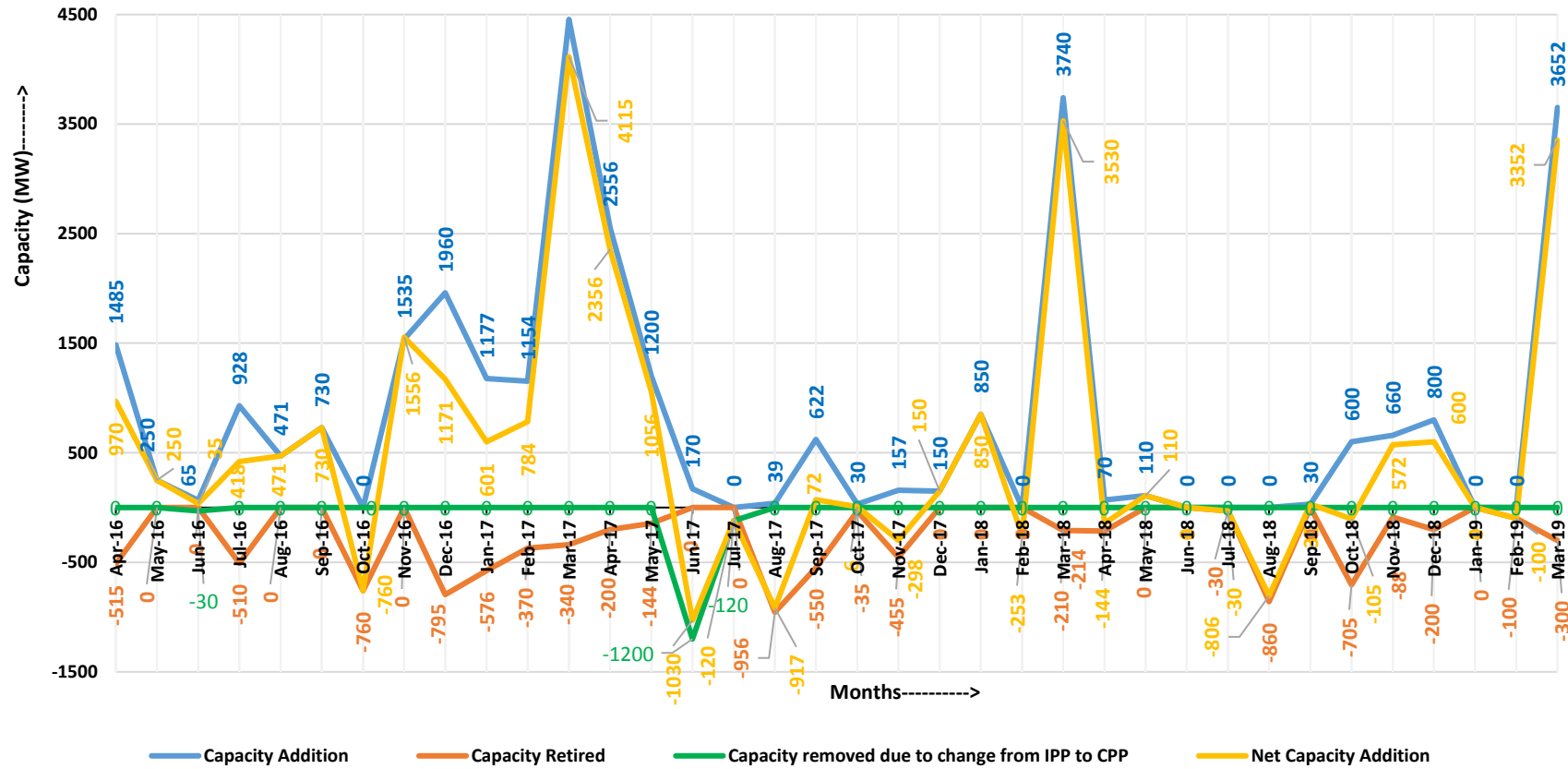
Trends of New Capacity Addition, Capacity Retired, Capacity removed due to change from IPP to CPP and Net Capacity Addition
