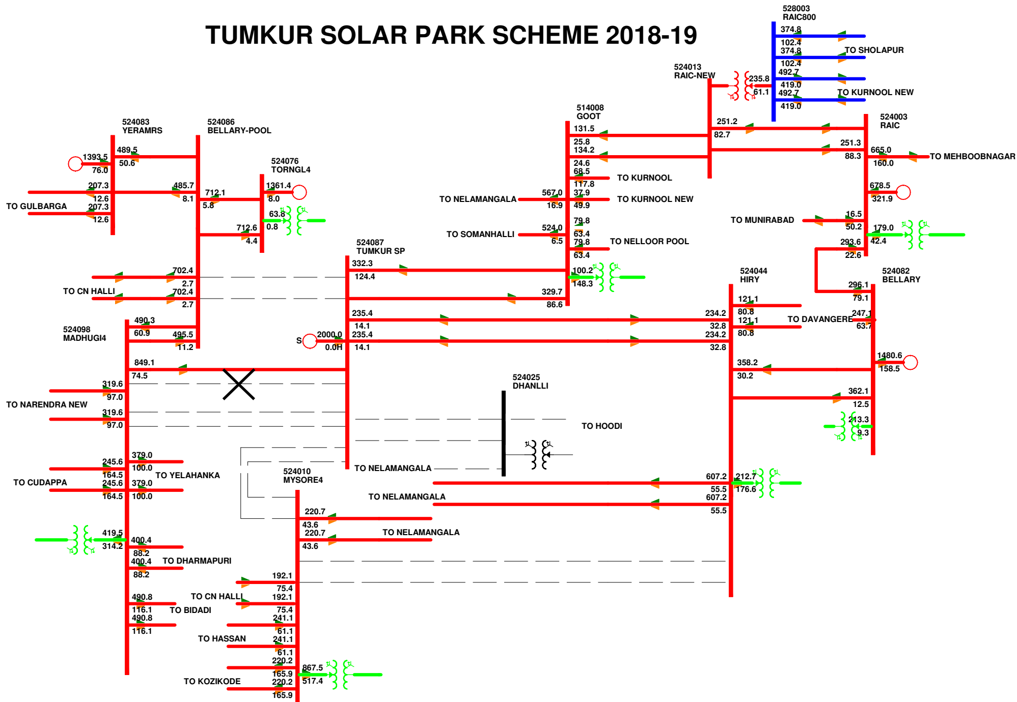
Outage of One Ckt of Tumkur -Madhugiri D/c
