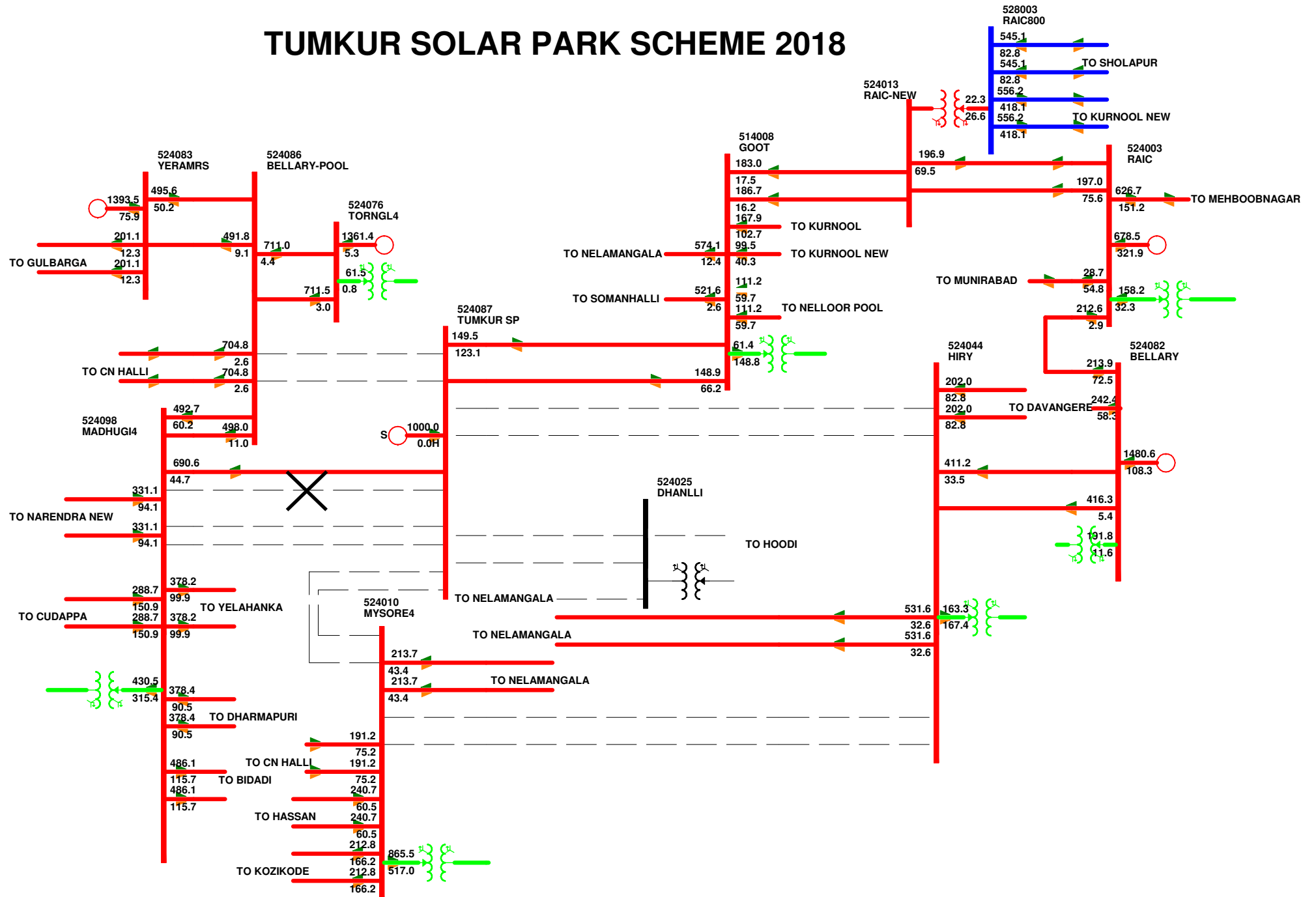
Ph-1 : Outage Of One Ckt of Tumkur-Madhugiri D/c
