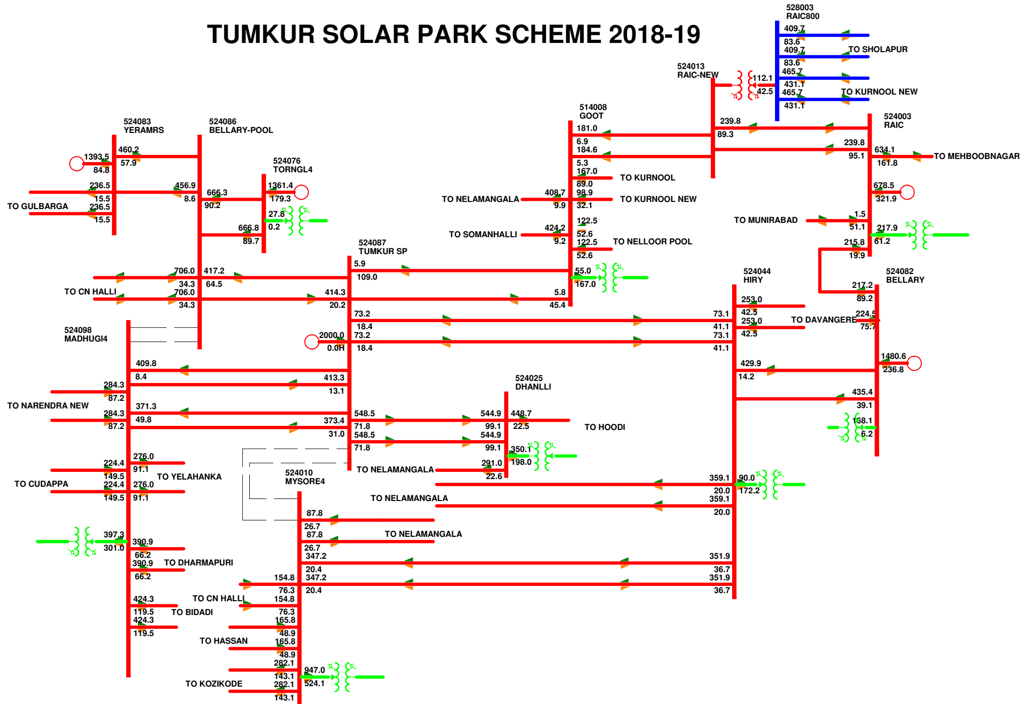
Base Case Ph-2 (2000 MW) :With Full Transmission System
