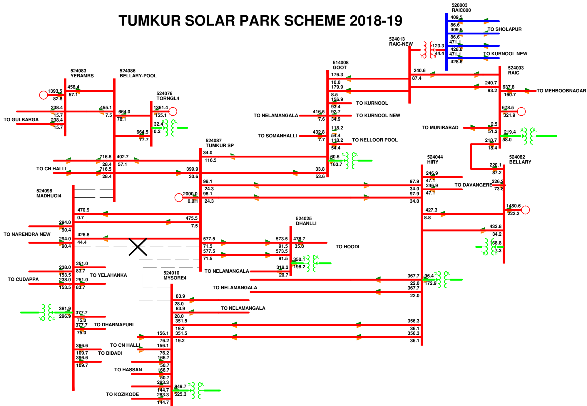
Outage of 1 Ckt of Tumkur Madhugiri D/c Quad Line
