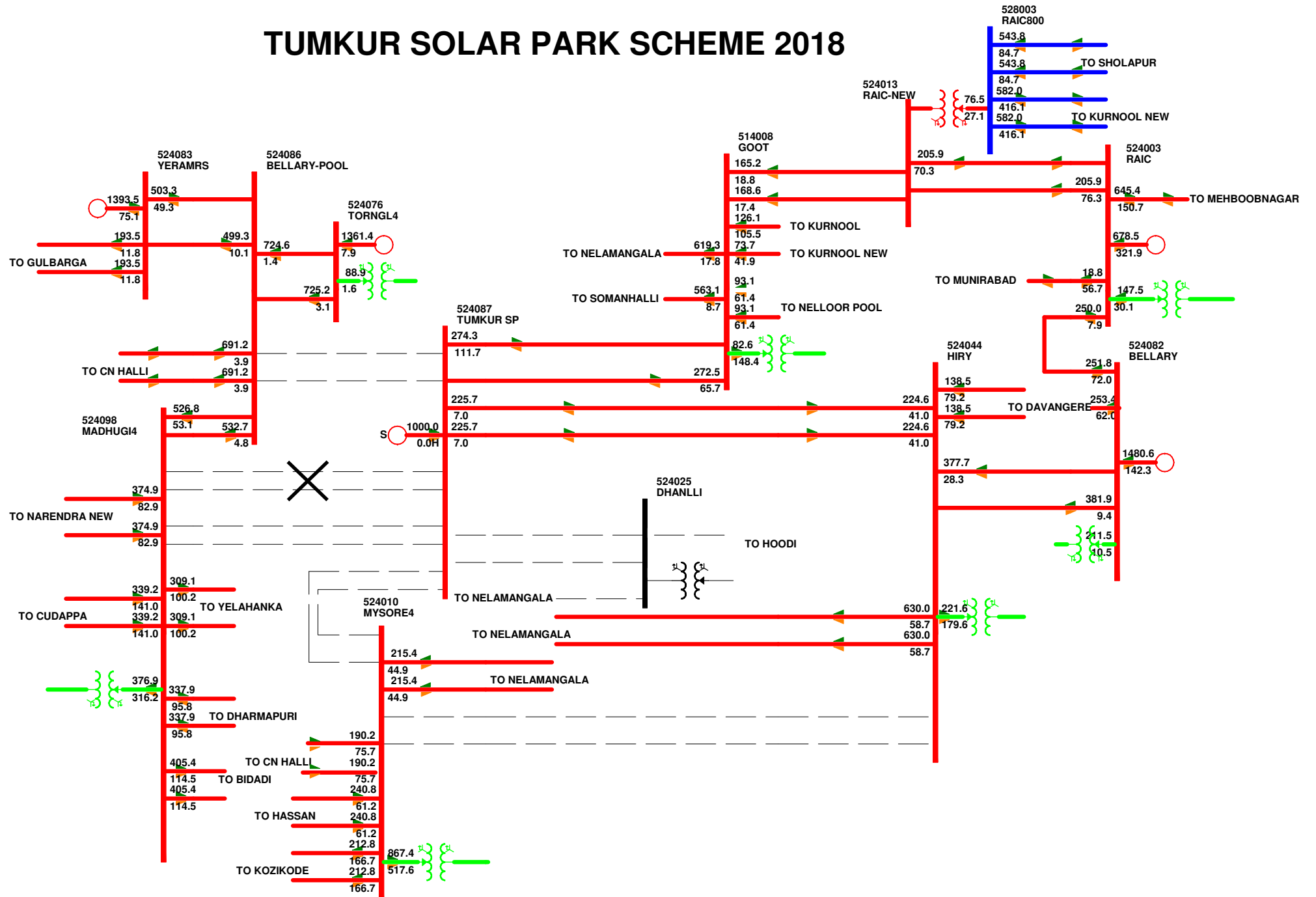
Ph-1 : Outage Of Both Ckts of Tumkur-Madhugiri D/c
