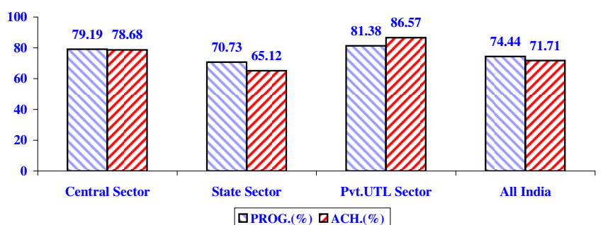
ALL INDIA PLANT LOAD FACTOR ( % ) DURING SEP.09
