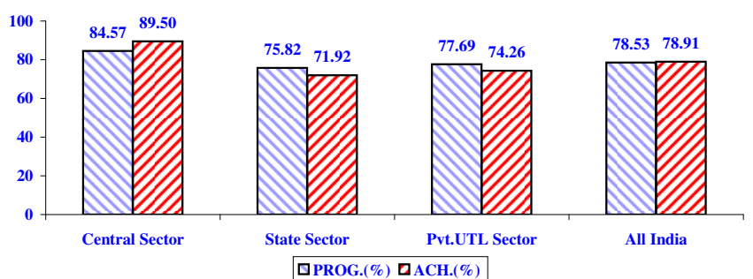
ALL INDIA PLANT LOAD FACTOR ( % ) DURING DEC.09
