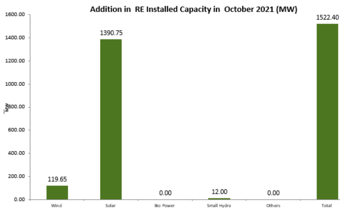
Figure 4: Source wise addition in RE Installed Capacity in October 21
