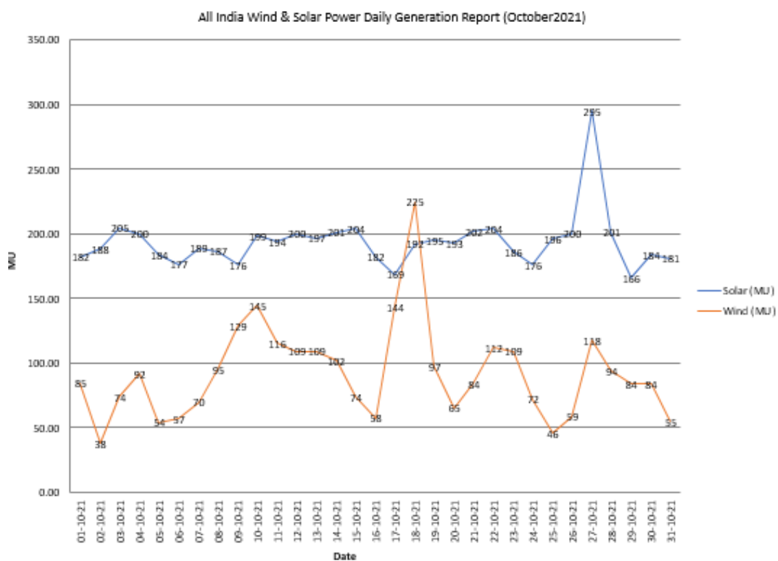
Figure 19 Daily Solar and wind Power Generation trend in the month of October -21
