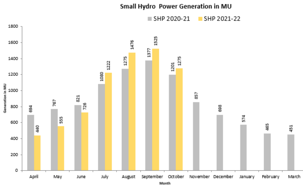
Figure 17: Monthly Small Hydro Power Generation (2021-22 Up to October -21)
