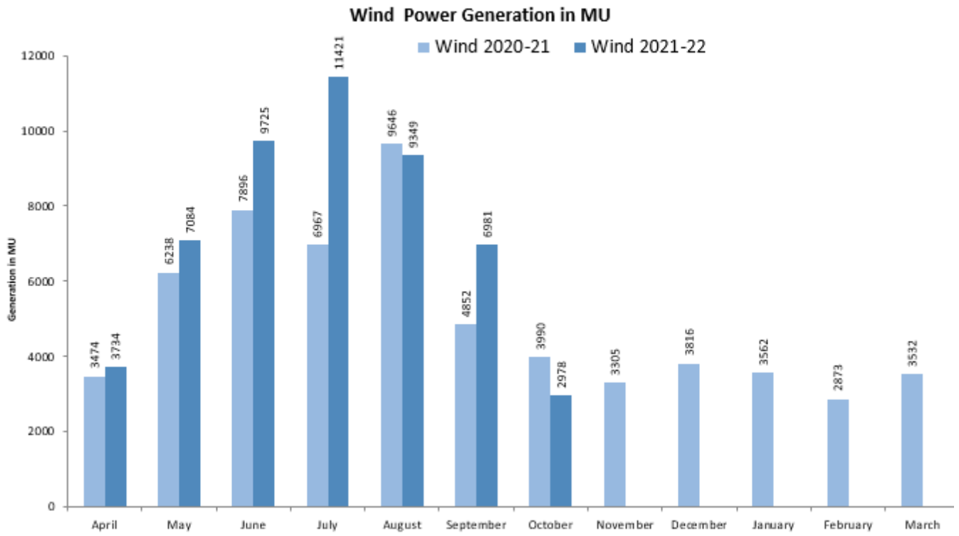
Figure 13 :Monthly Wind Power Generation (2021-22 Up to October -21)
