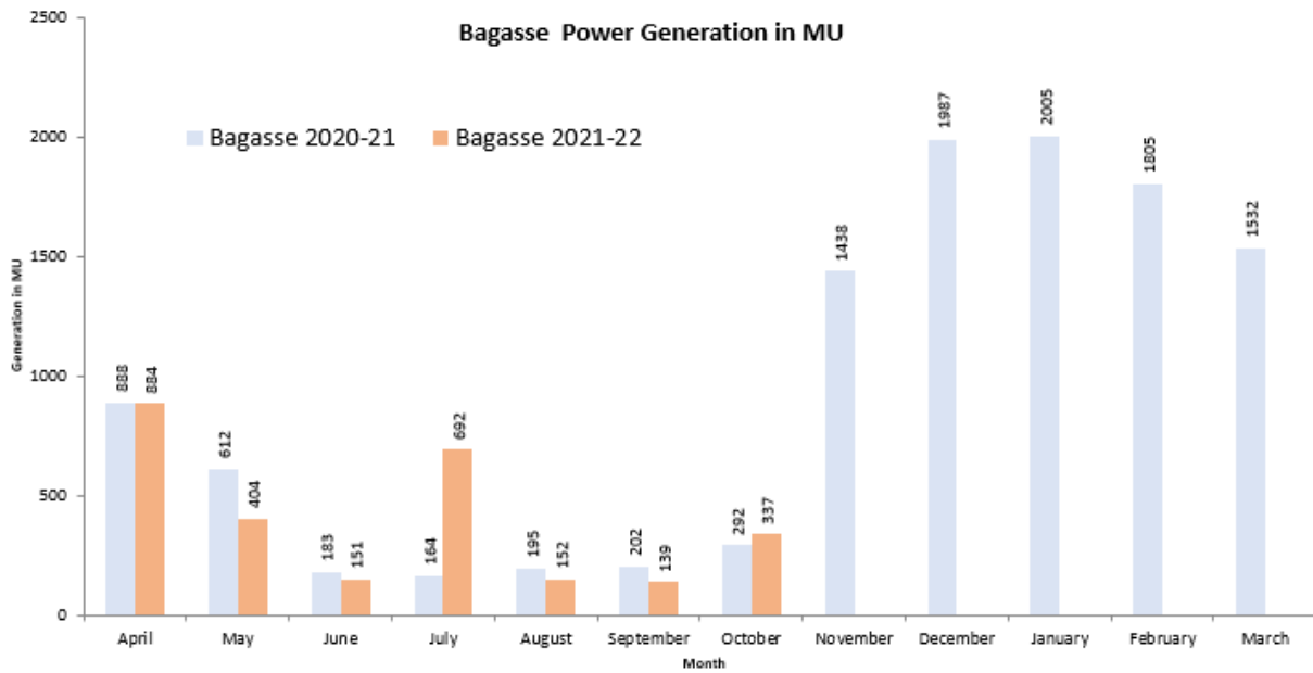
Figure 16 : Monthly Bagasse Power Generation (2021-22 Up to October -21)
