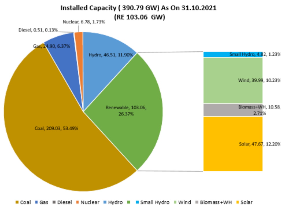
Figure 3 Installed Capacity in India as on 31.10.2021
