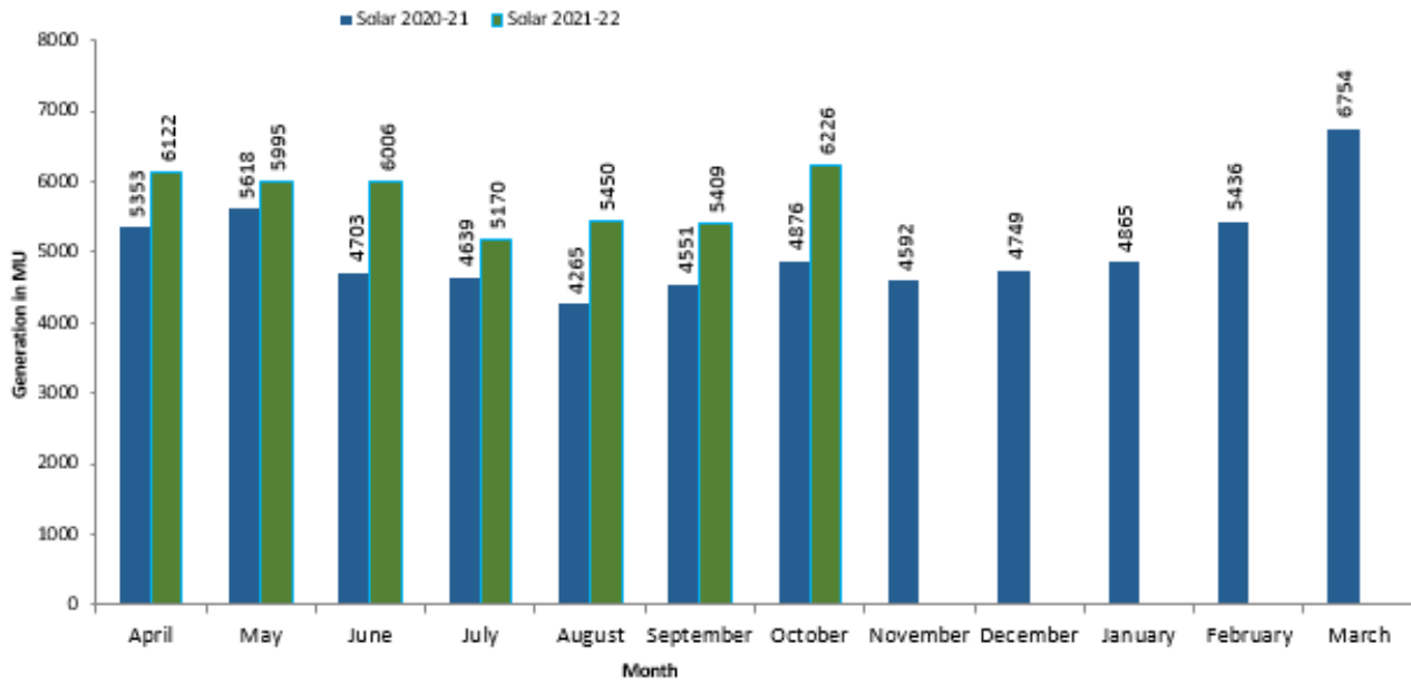
Figure 14: Monthly Solar Power Generation (2021-22 Up to October -21)
