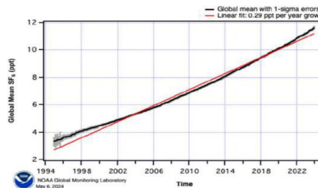
Atmospheric concentration of SF 6
