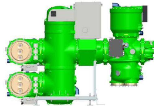
Typical GIS Switchgear filled with g^3 gas
