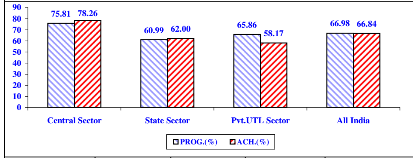
ALL INDIA PLANT LOAD FACTOR ( % ) DURING JULY.12
