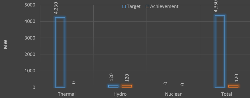
Capacity Addition Targets/Achievements during the Month of Oct-2022
