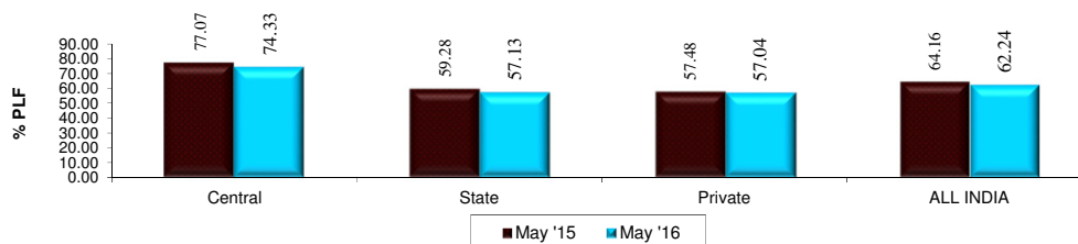
Sector-Wise Plant Load Factor for May, 2015 and May, 2016
