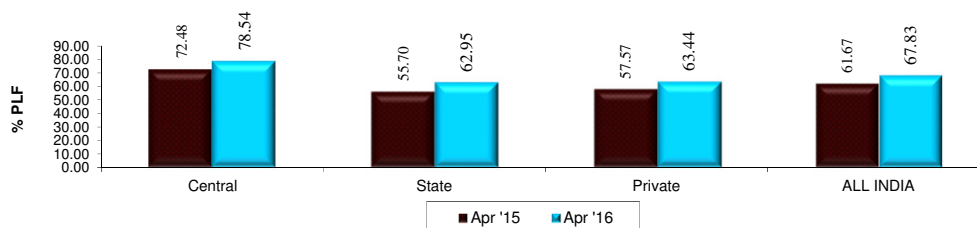
Sector-Wise Plant Load Factor for Apr 2015 and Apr 2016
