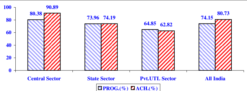
ALL INDIA PLANT LOAD FACTOR ( % ) DURING JANUARY.11
