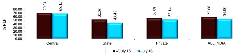
Sector-Wise Plant Load Factor for July, 2015 and July, 2016
