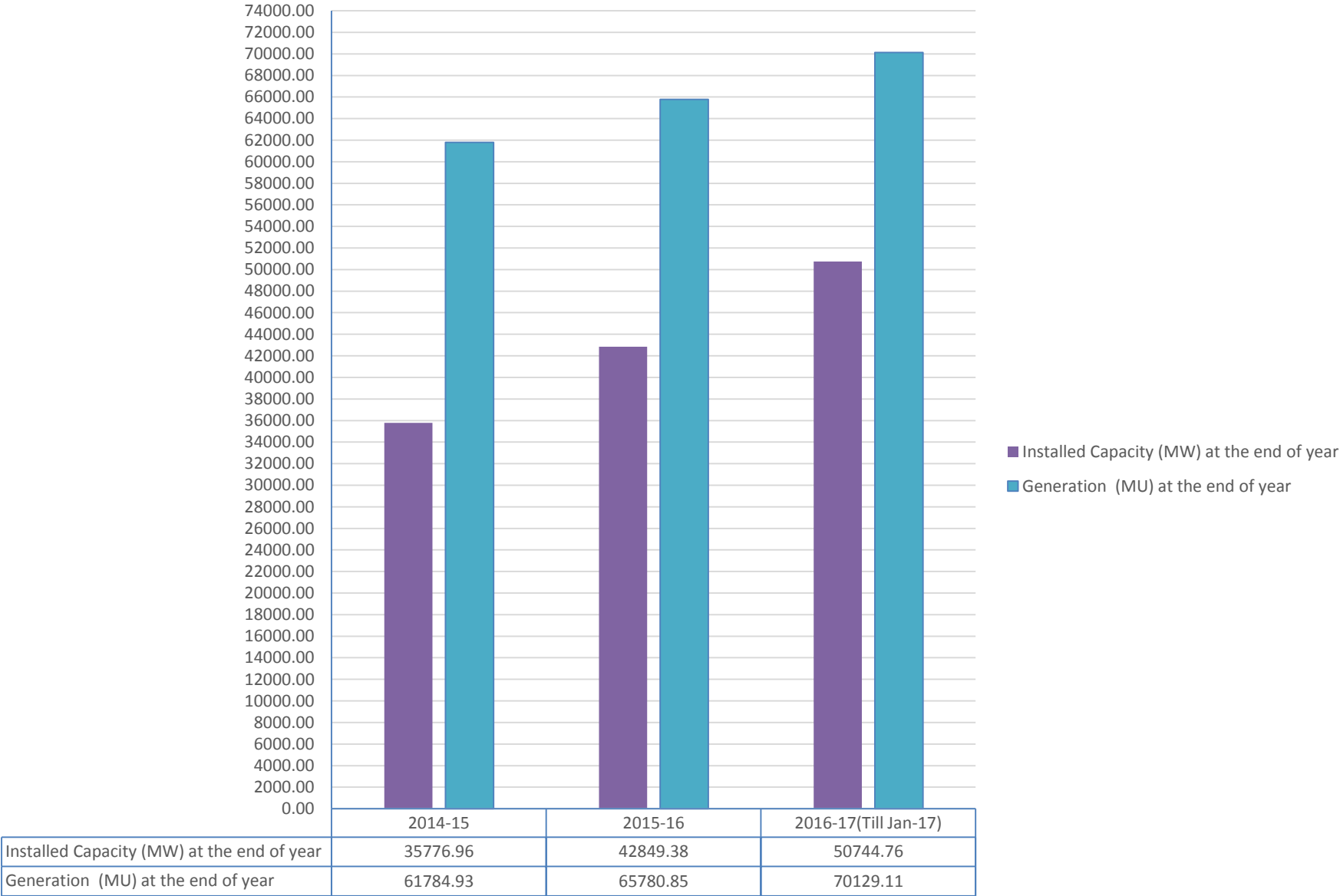
Installed Capacity Vs Generation
