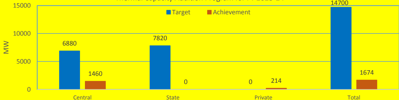
Thermal Capacity Addition Program for FY 2023-24
