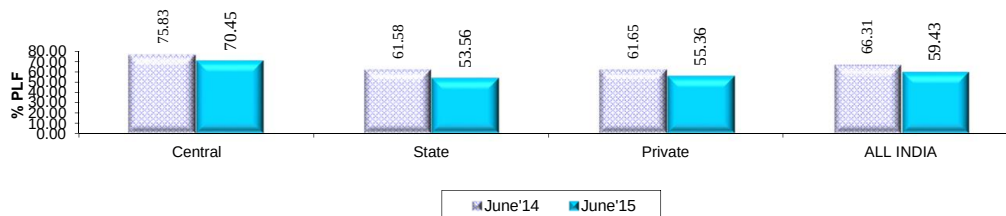
Sector-Wise Plant Load Factor for June '14 and June '15
