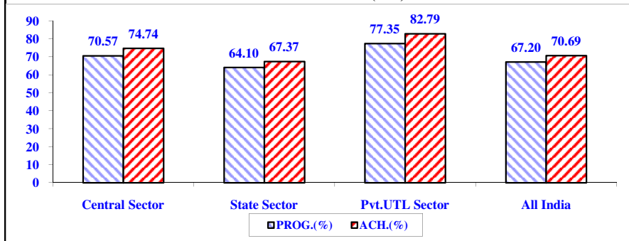
ALL INDIA PLANT LOAD FACTOR ( % ) DURING OCTOBER. 11
