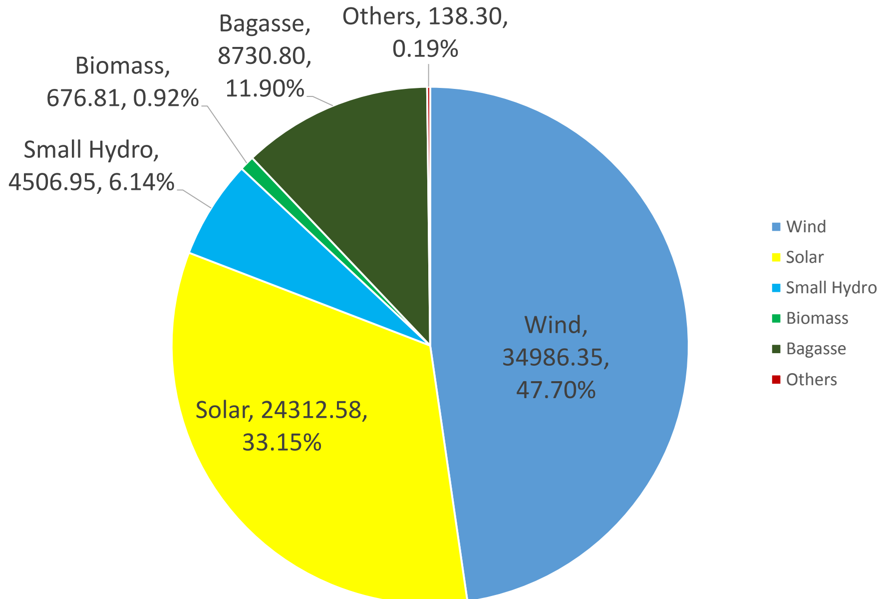
Source wise breakup of RE Installed Capacity till October 2018
