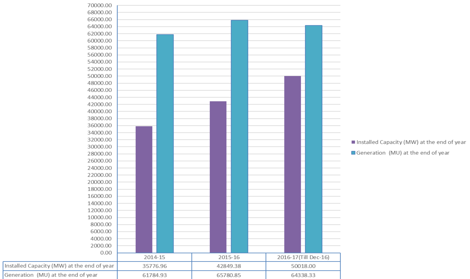
Installed Capacity Vs Generation for all Renewable Energy Sources
