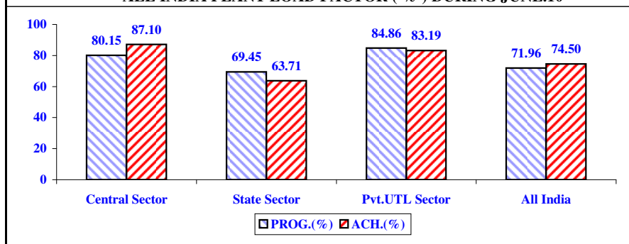
ALL INDIA PLANT LOAD FACTOR ( % ) DURING JUNE.10
