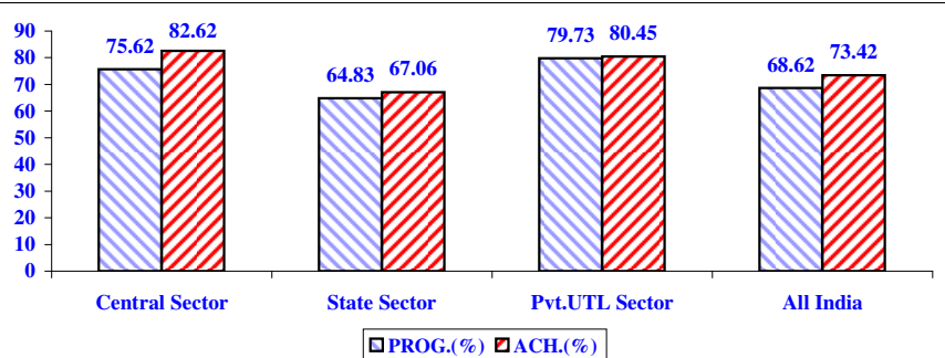
ALL INDIA PLANT LOAD FACTOR ( % ) DURING JUNE. 11
