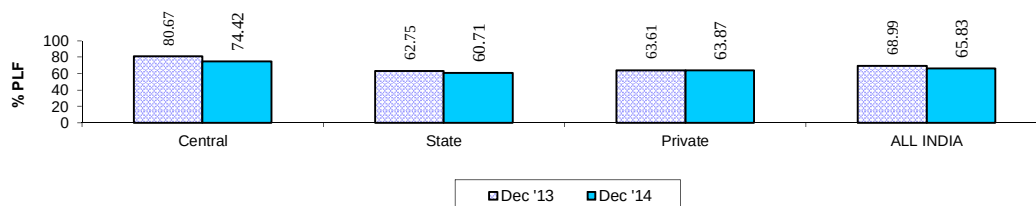
Sector-Wise Plant Load Factor for December 2013 and December 2014
