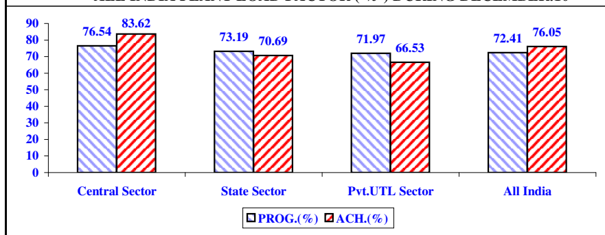
ALL INDIA PLANT LOAD FACTOR ( % ) DURING DECEMBER.10
