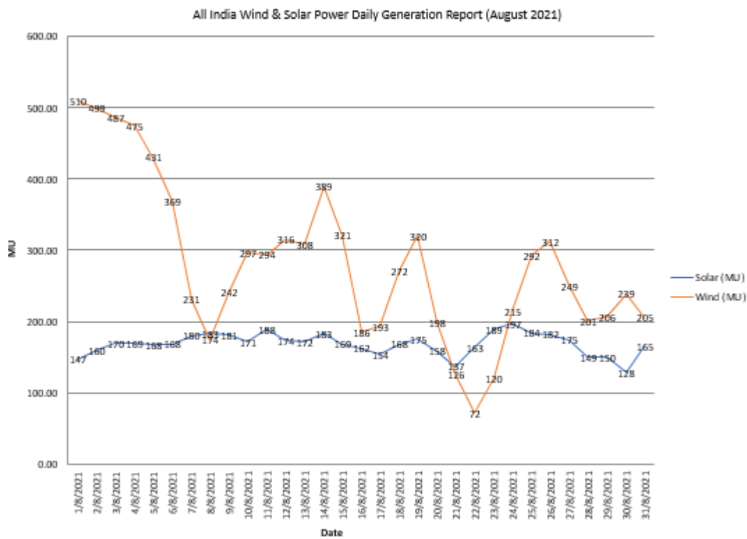
Figure 19 Daily Solar and wind Power Generation trend in the month of August -21
