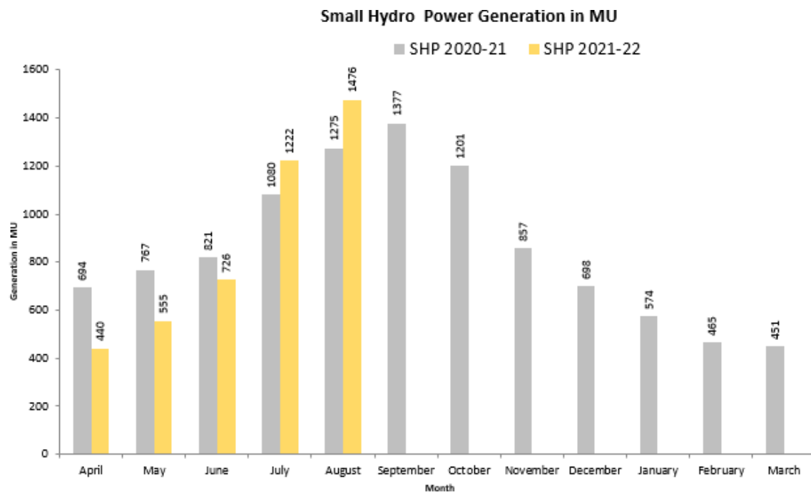
Figure 17 Monthly Small Hydro Power Generation (2021-22 Up to August -21)
