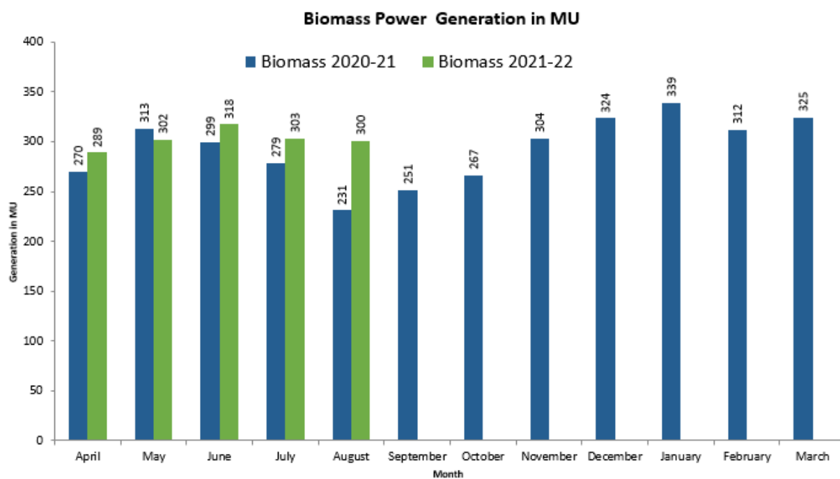
Figure 15 Monthly Biomass Power Generation (2021-22 Up to August -21)
