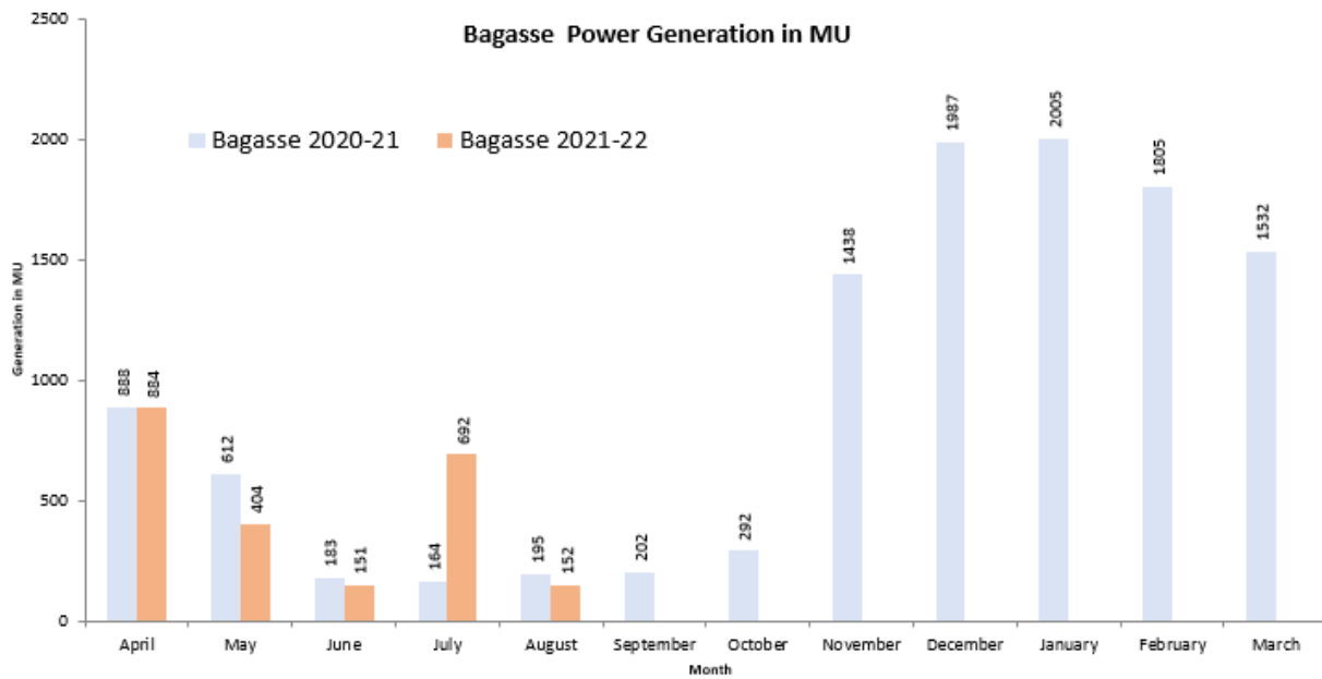
Figure 16 Monthly Bagasse Power Generation (2021-22 Up to August -21)
