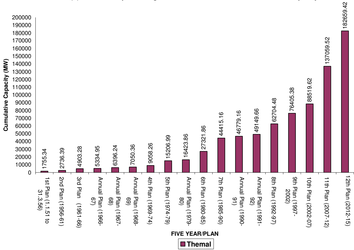
9(b) Bar Chart representing Plan-Wise Growth of Thermal Installed Capacity
