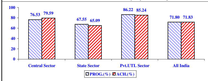
ALL INDIA PLANT LOAD FACTOR ( % ) DURING JULY.09
