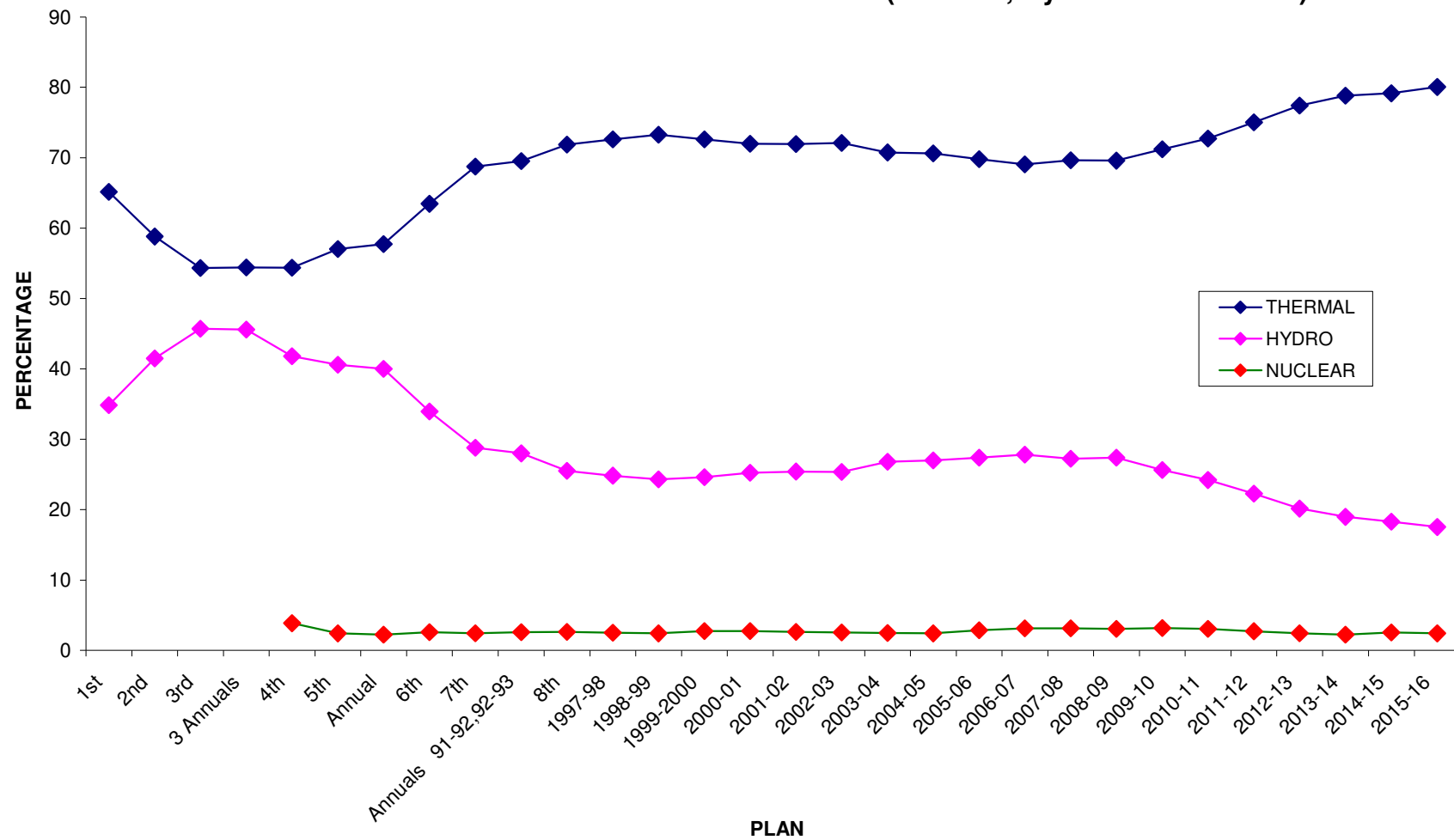
8b. TREND OF CAPACITY ADDITION AS % OF TOTAL(Thermal, Hydro & Nuclear Mix)
