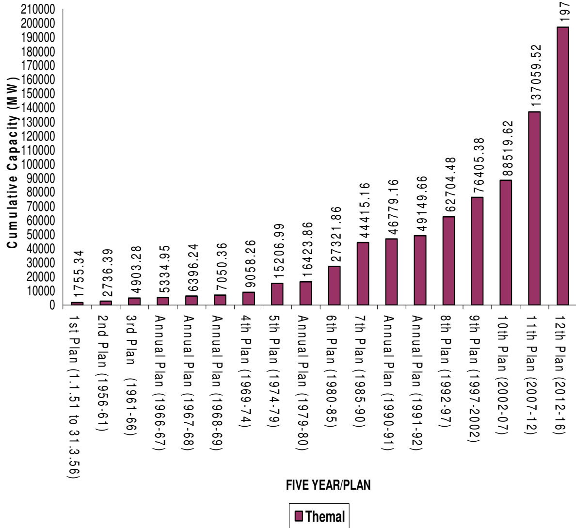
9(b) Bar Chart representing Plan-Wise Growth of Thermal Installed Capacity
