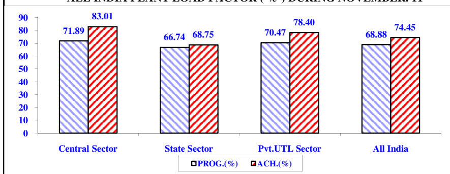
ALL INDIA PLANT LOAD FACTOR ( % ) DURING NOVEMBER. 11
