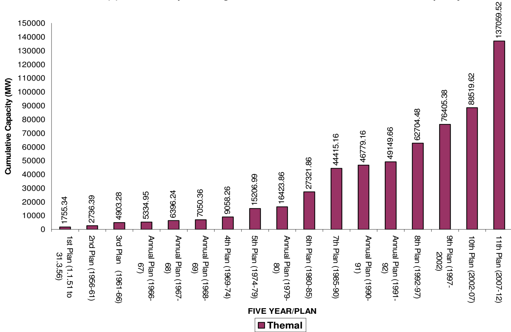
11(a) Bar Chart representing Plan-Wise Growth of Thermal Installed Capacity
