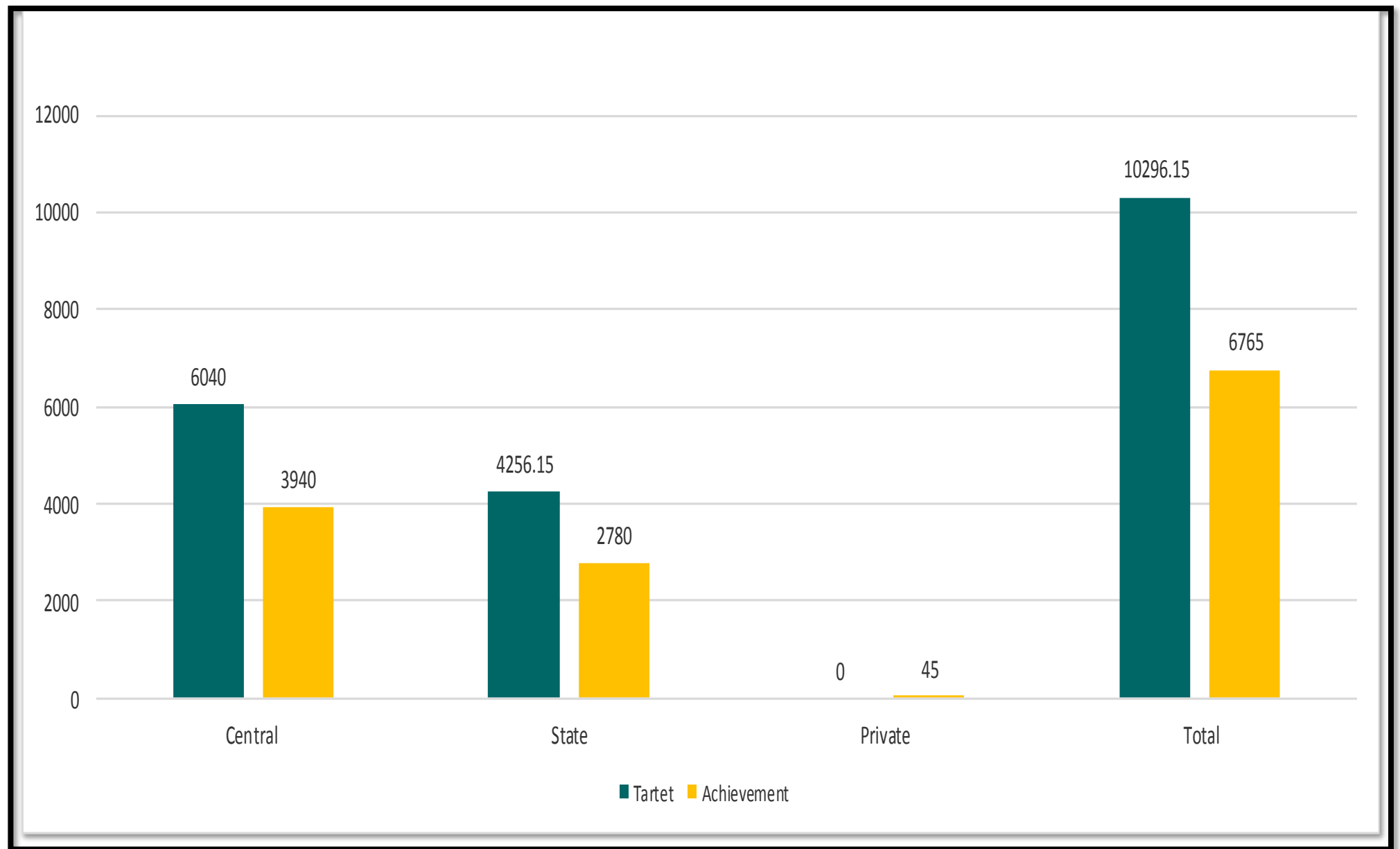
Bar Chart showing Thermal Capacity Addition Target/Achievement during the year 2019-20(MW)
