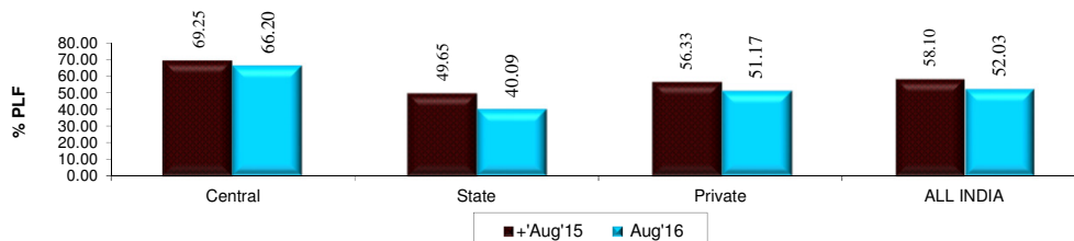
Sector-Wise Plant Load Factor for Aug, 2015 and Aug, 2016
