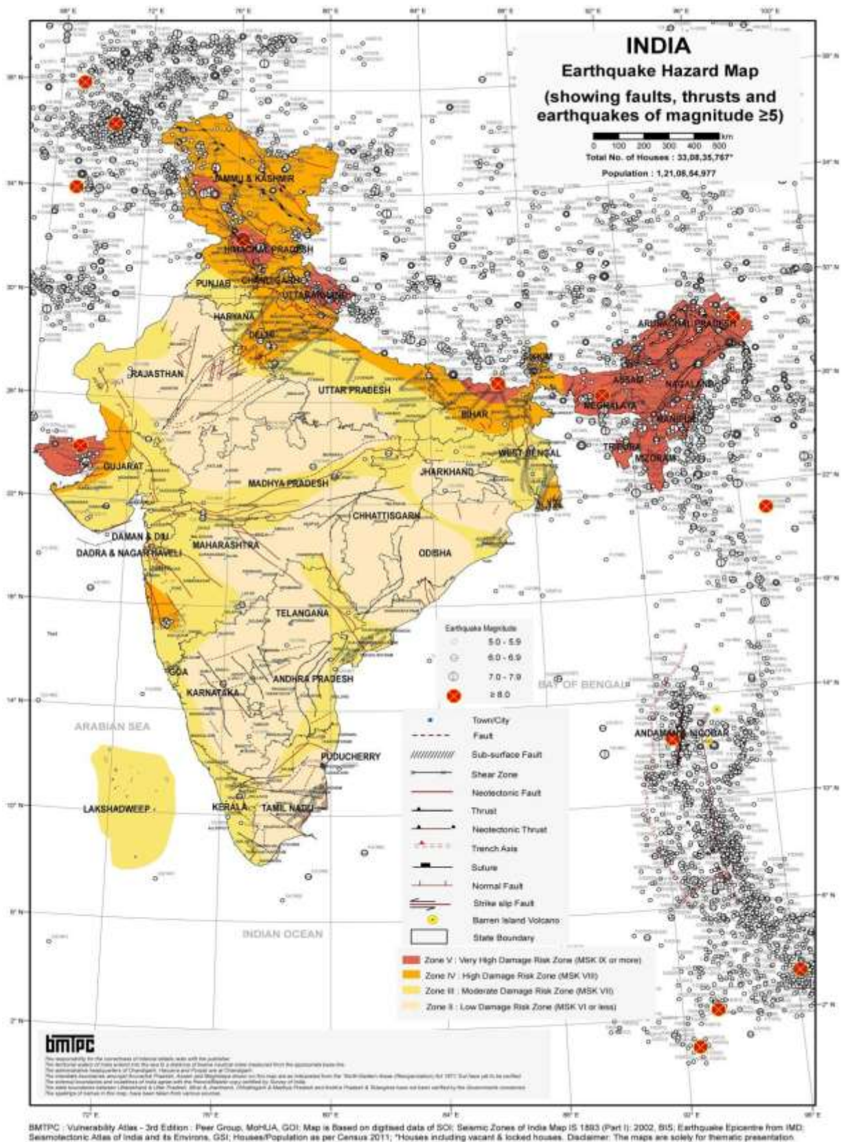
Earthquake Hazard Map of India
