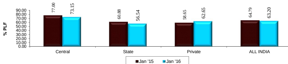
Sector-Wise Plant Load Factor for January 2015 and January 2016
