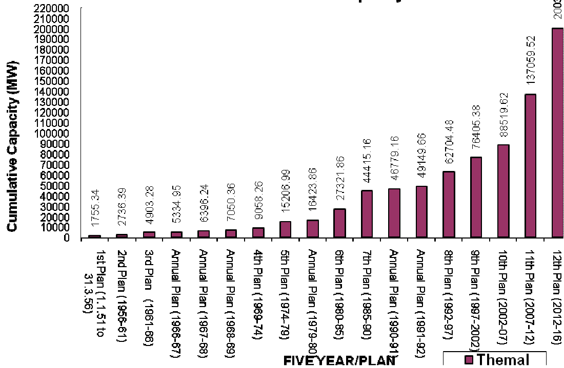
9(b) Bar Chart representing Plan-Wise Growth of Thermal Installed Capacity
