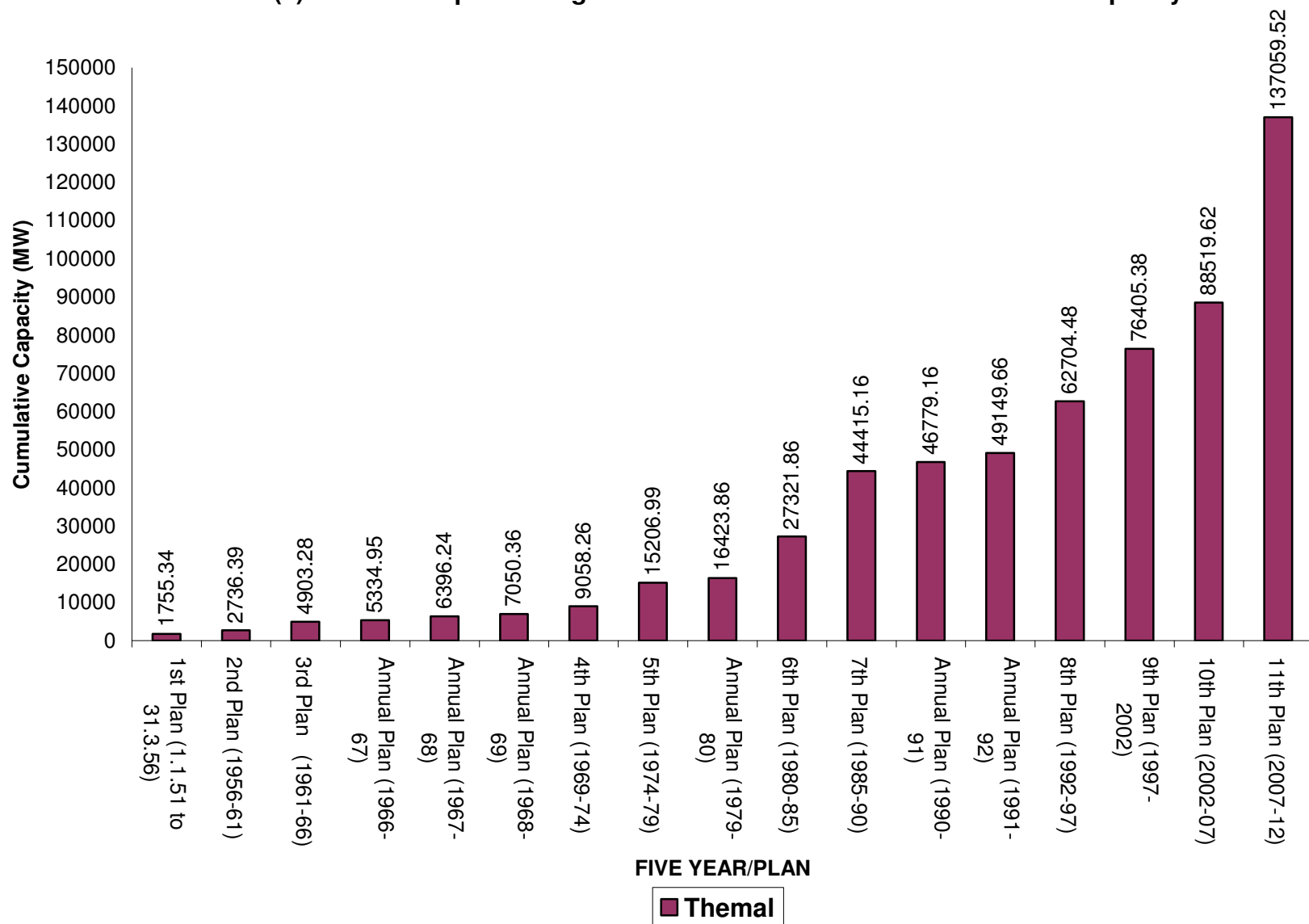
11(a) Bar Chart representing Plan-Wise Growth of Thermal Installed Capacity
