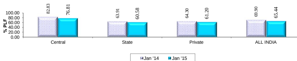
Sector-Wise Plant Load Factor for January 2014 and January 2015
